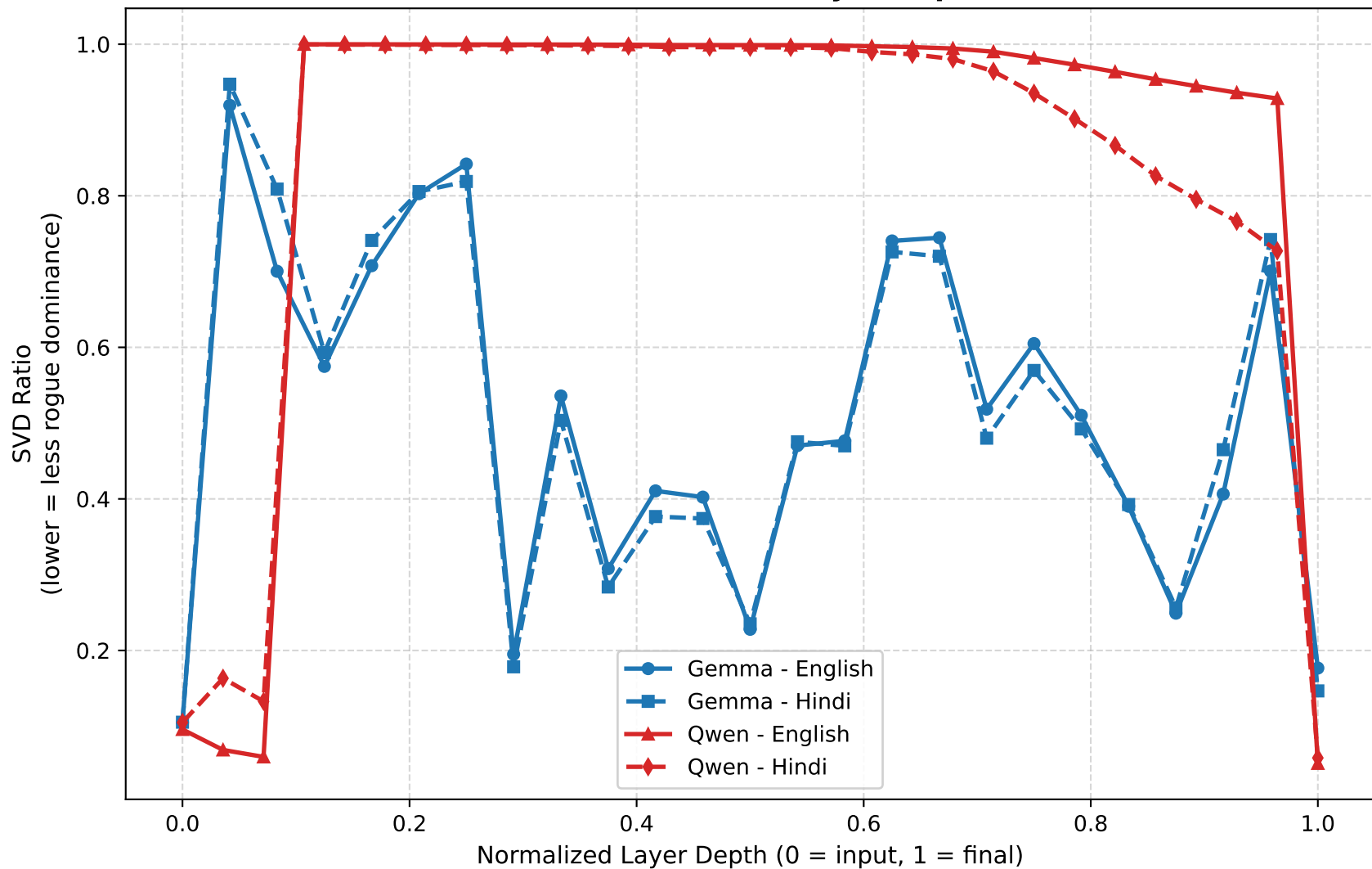
SVD Ratio across Layer Depth
