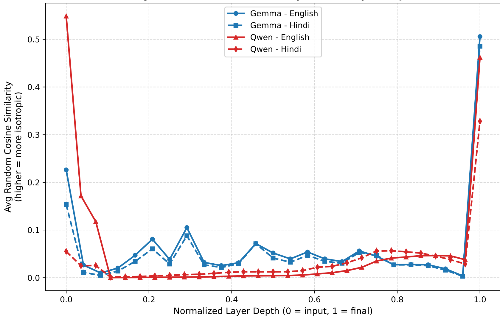
Avg Random Cosine Similarity across Layer Depth
