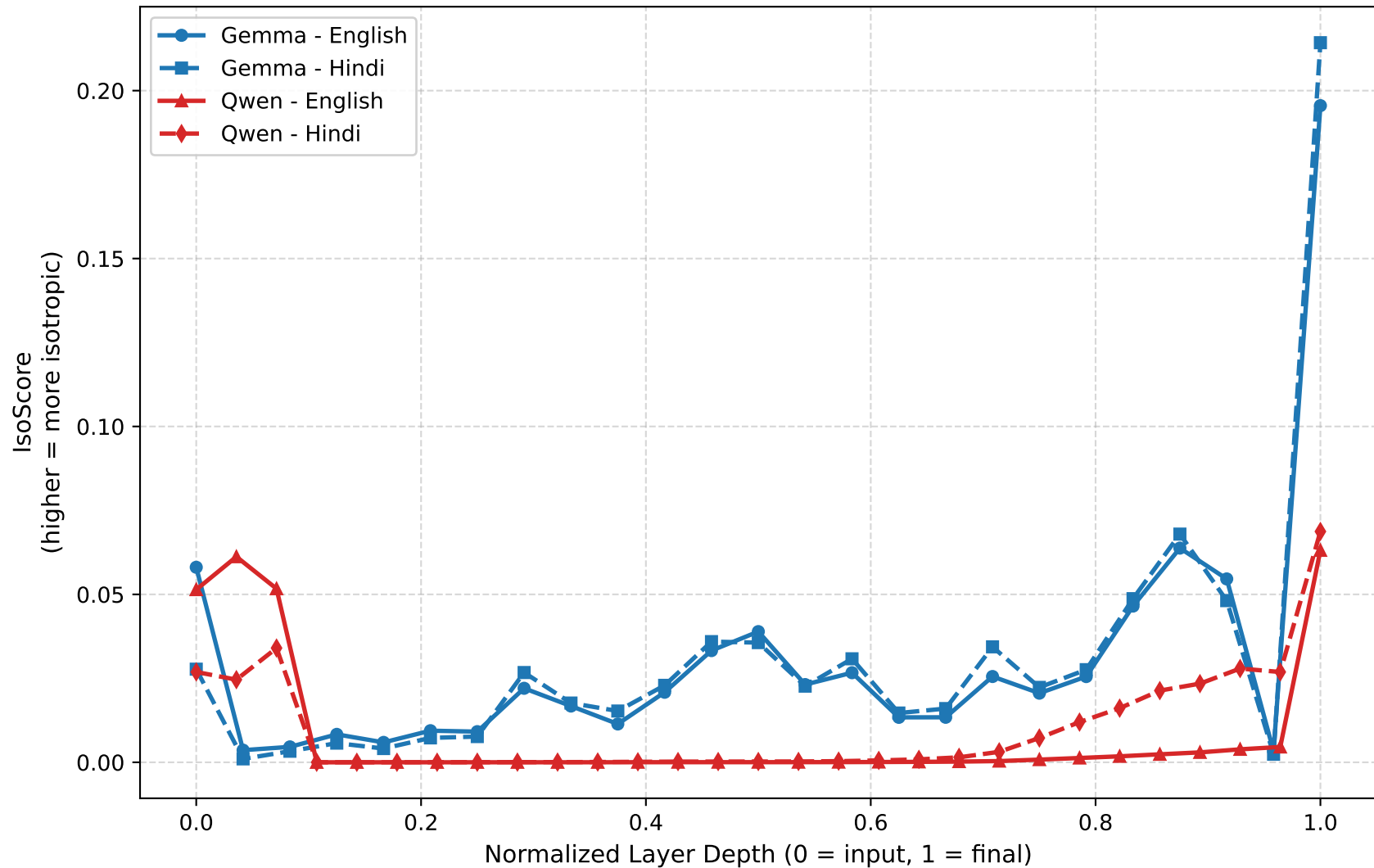
IsoScore across Layer Depth
