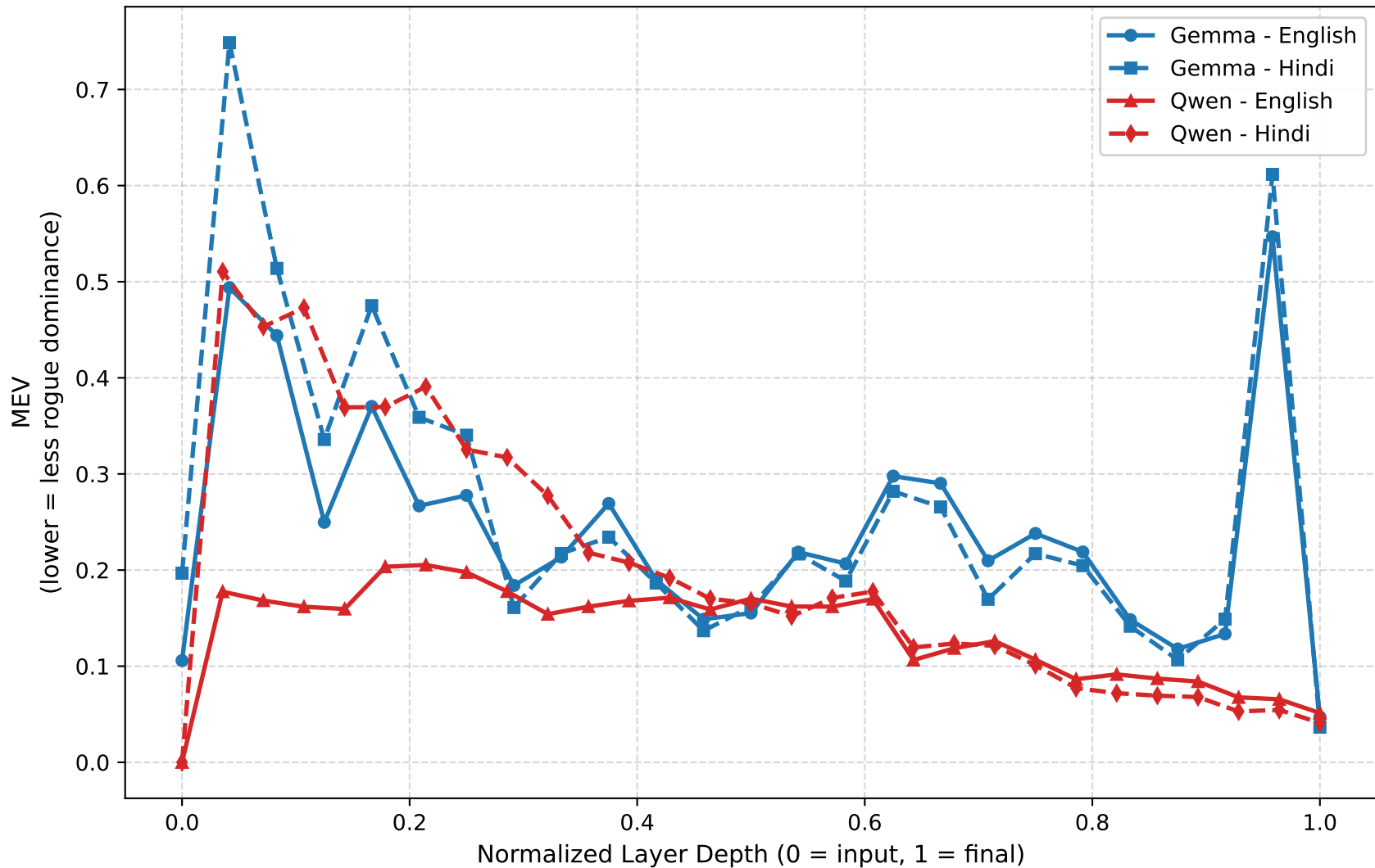
MEV across Layer Depth
