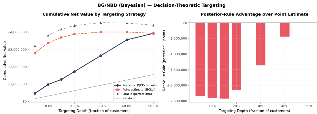
Figure 5.10: Decision-theoretic targeting for the Bayesian model at the headline cost of £20. Left: cumulative net value by strategy and depth. Right: the net-value advantage of the posterior rule over the point estimate.
