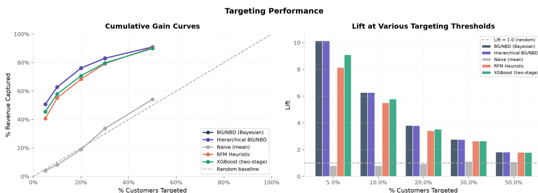
Figure 5.11: Cumulative-gain and lift curves for all models. Steeper early rise indicates better identification of high-value customers.
