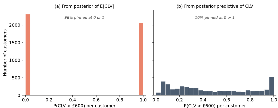
Figure 5.12: Distribution of the per-customer targeting probability P(\text{CLV} > £600) across all 4,522 customers. (a) Computed from the posterior of E[\text{CLV}] , the probability saturates: 96% of customers sit at 0 or 1. (b) Computed from the posterior predictive of realised CLV, it is graded and usable as a decision score. This is the saturation artefact that makes the expectation-based rule fail for mechanical reasons.
