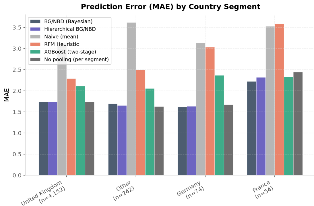
Figure 5.9: Per-country transaction MAE by model. Differences concentrated in the small segments (Germany, France, Other) test the partial-pooling hypothesis.
