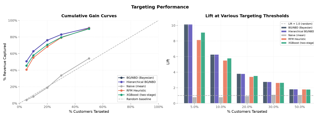
Figure 5.13: Cumulative-gain and lift curves for all models. Steeper early rise indicates better identification of high-value customers.
