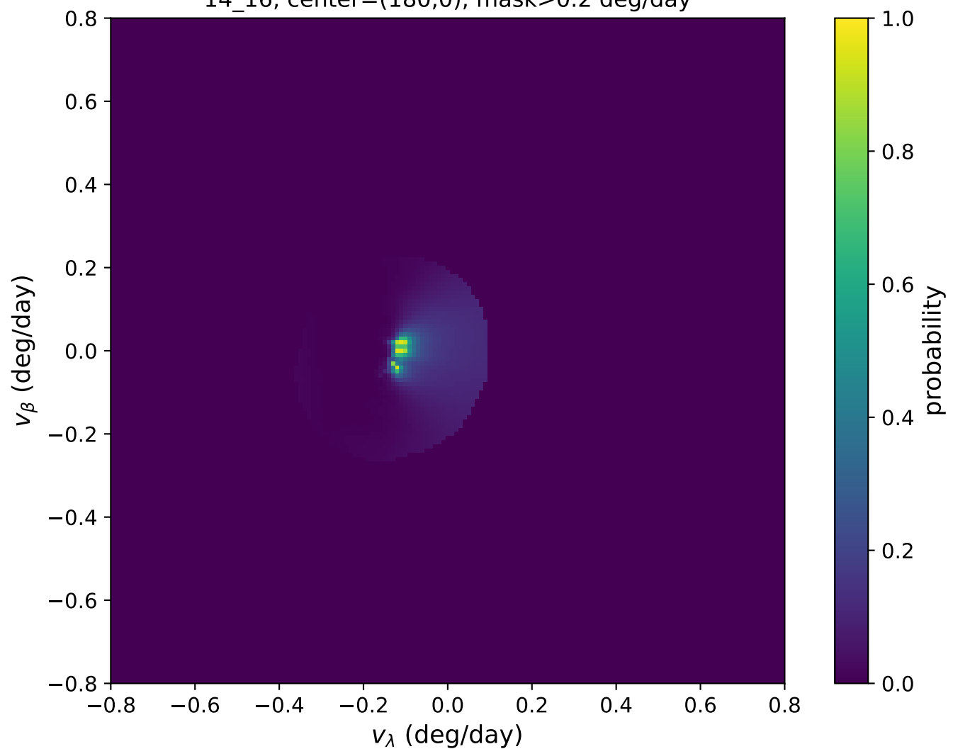
Trojans: cloned/downweighted probability 14_16, center=(180,0), mask>0.2 deg/day
