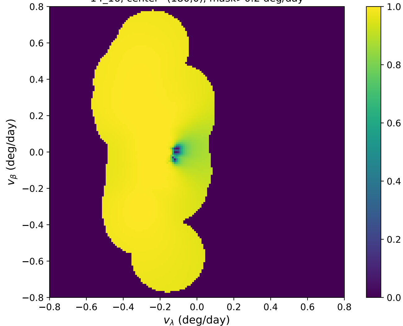
TNO: cloned/downweighted probability 14_16, center=(180,0), mask>0.2 deg/day
