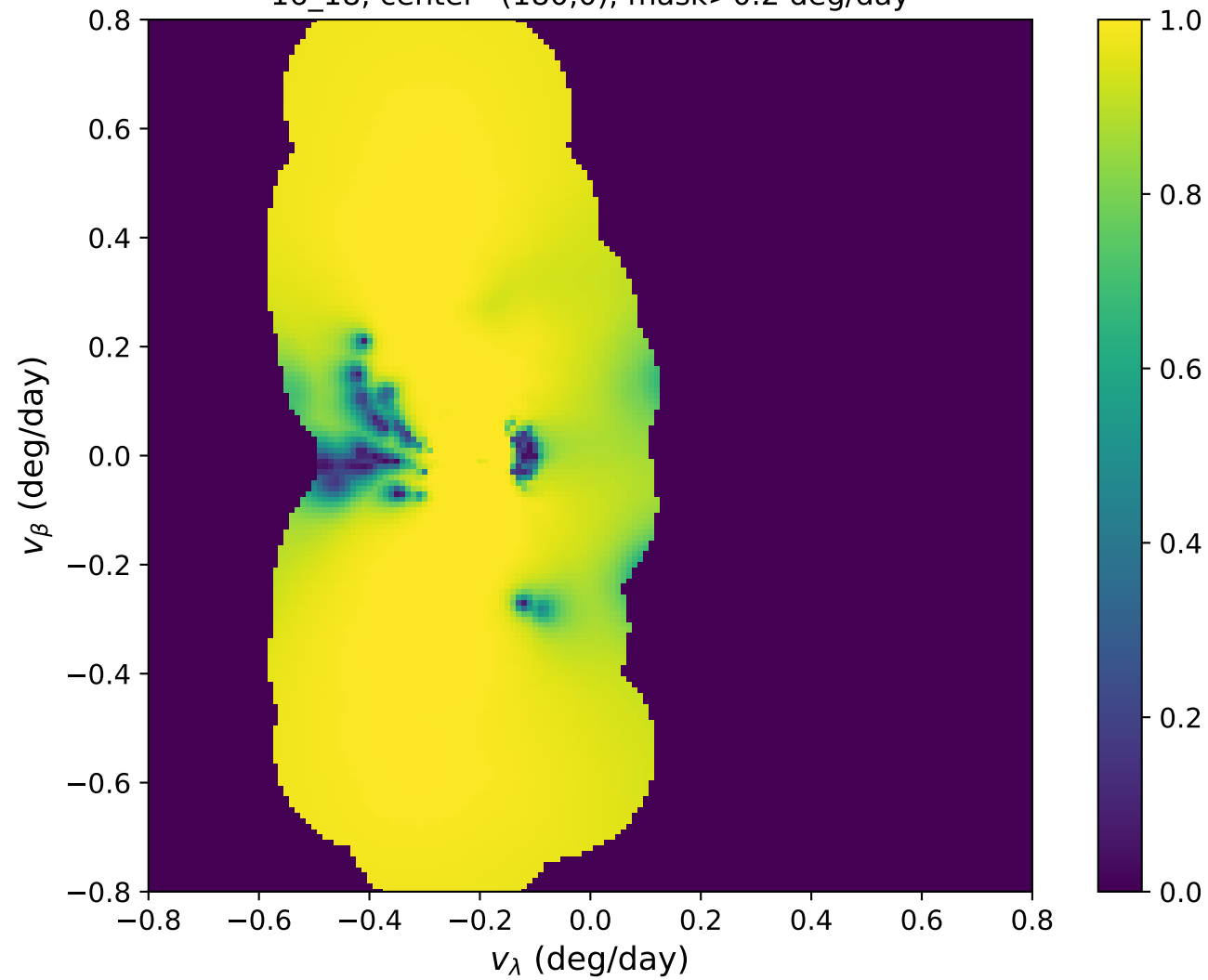
TNO: cloned/downweighted probability 16_18, center=(180,0), mask>0.2 deg/day
