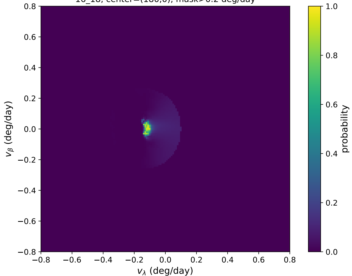
Trojans: cloned/downweighted probability 16_18, center=(180,0), mask>0.2 deg/day
