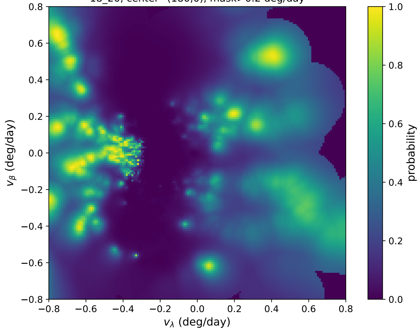
Trojans: cloned/downweighted probability 18_20, center=(180,0), mask>0.2 deg/day
