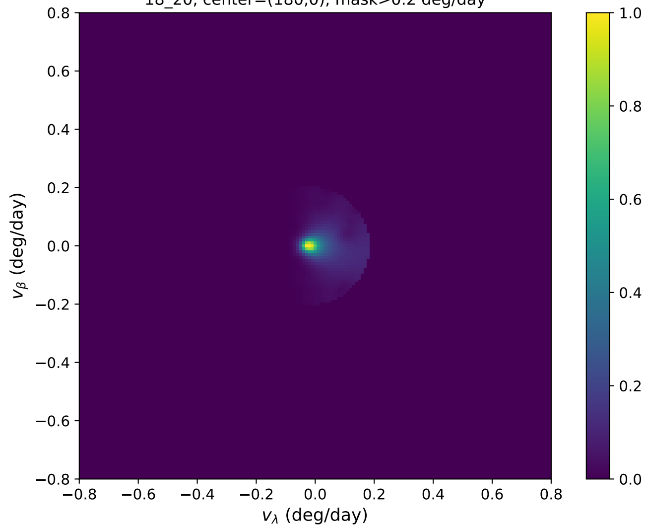
TNO: cloned/downweighted probability 18_20, center=(180,0), mask>0.2 deg/day
