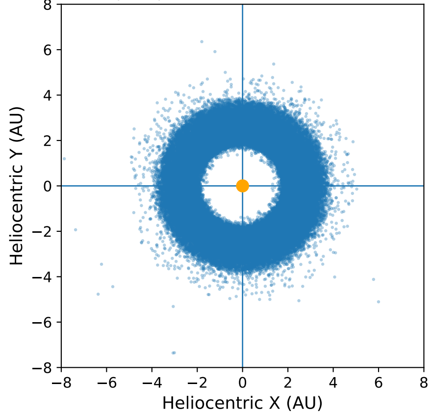
MBA ( |\beta| < 3.0^\circ ): heliocentric ecliptic X-Y
