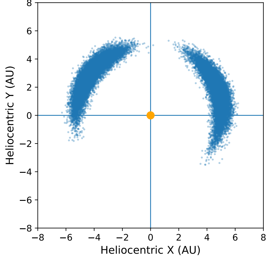
Jupiter Trojans ( |\beta| < 3.0^\circ ): heliocentric ecliptic X-Y
