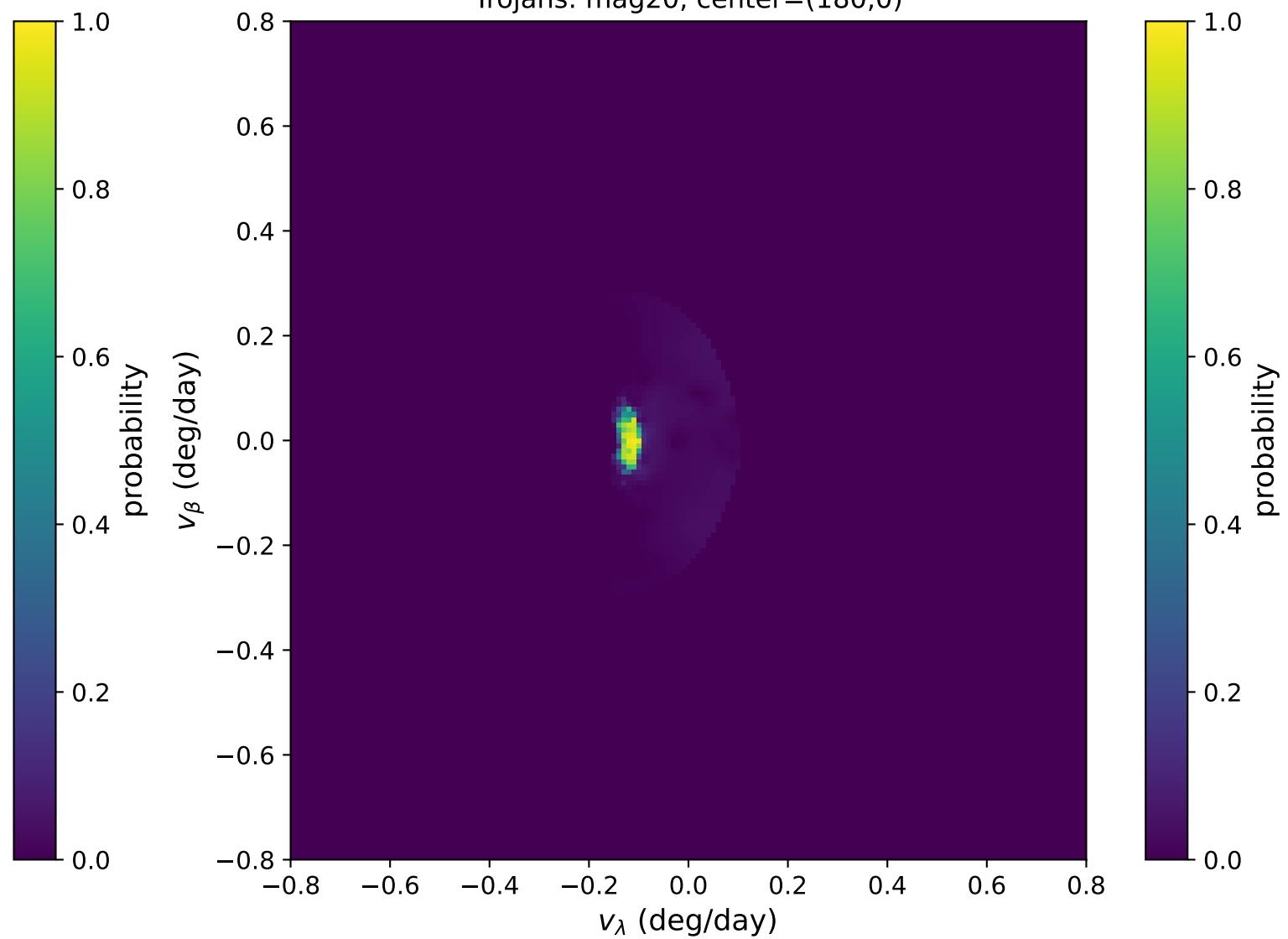
Trojans: mag20, center=(180,0)
