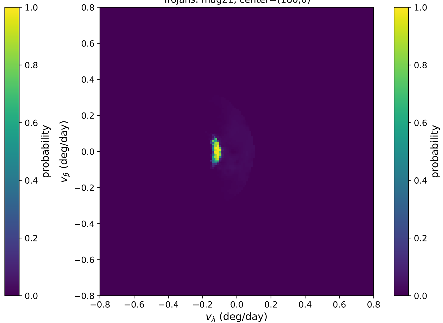
Trojans: mag21, center=(180,0)
