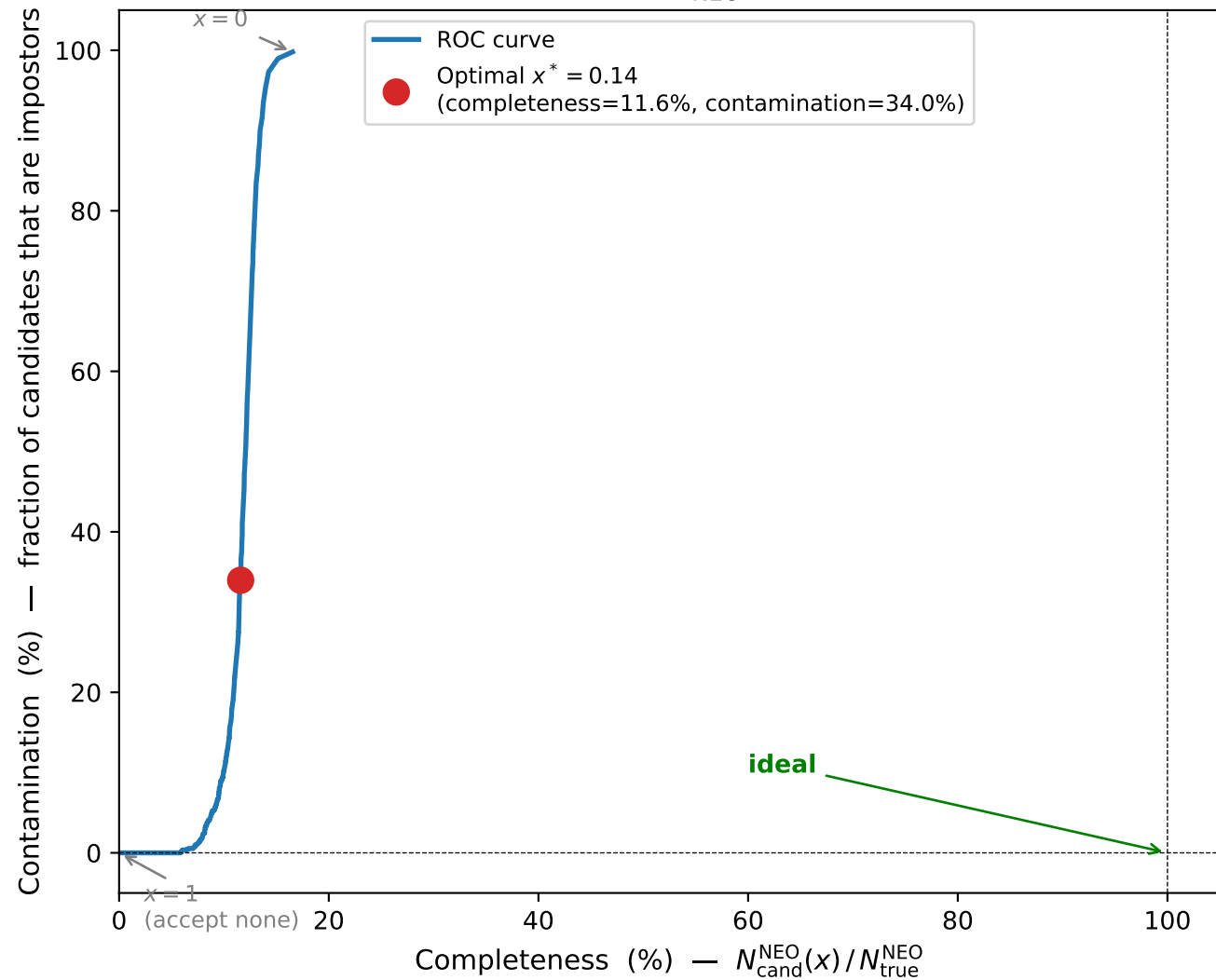
ROC Curve — P_{\text{NEO}} classifier
