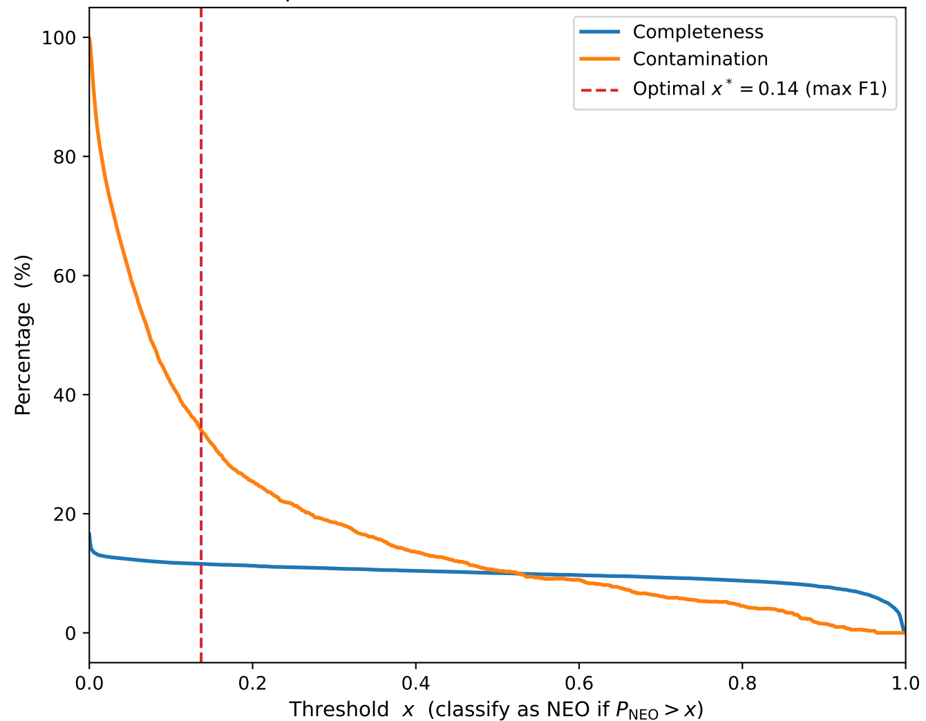
Completeness & Contamination vs threshold
