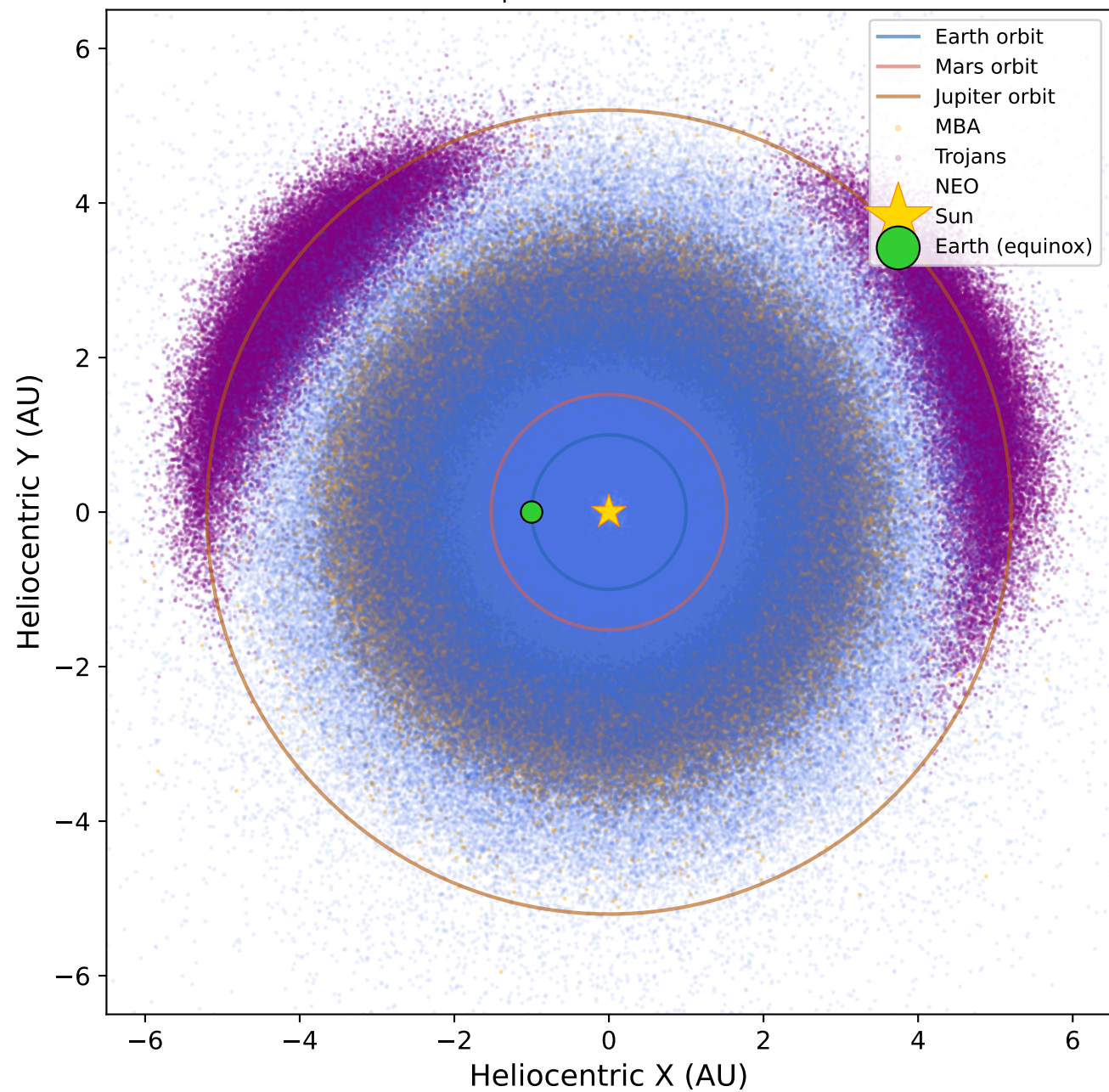
Heliocentric ecliptic plane — inner solar system (2025-03-21, K|M cloned orbits, no beta filter)
