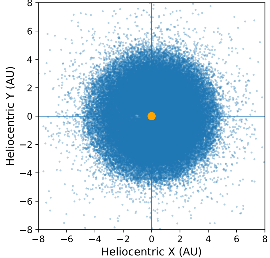
NEO ( |\beta| < 3.0^\circ ): heliocentric ecliptic X-Y
