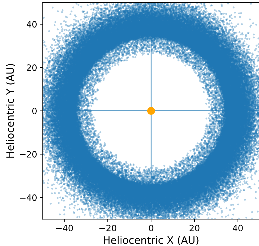
TNO ( |\beta| < 3.0^\circ ): heliocentric ecliptic X-Y
