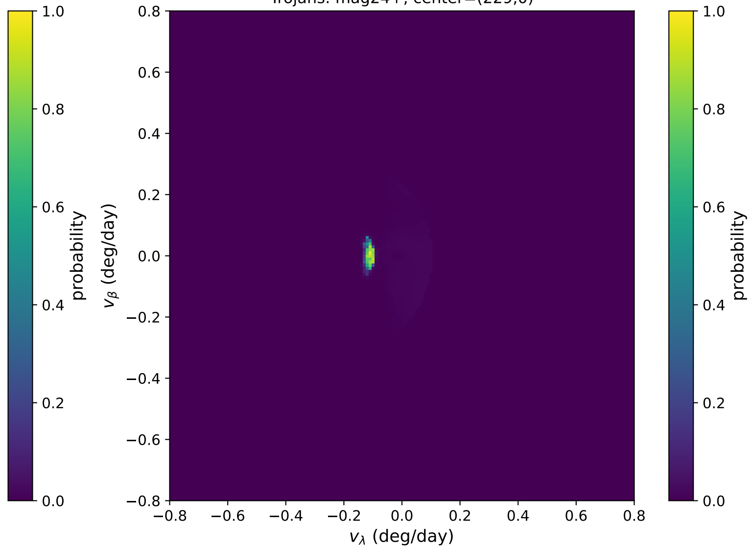
Trojans: mag24+, center=(229,0)
