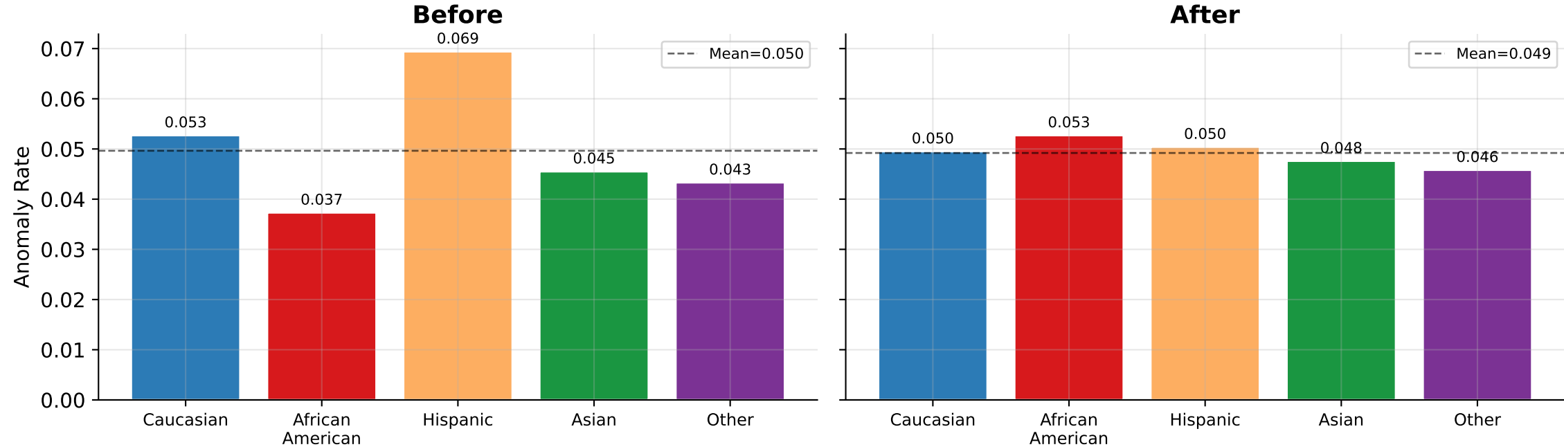
Figure 5: Per-Group Anomaly Rates Before vs After Debiasing (IF)
