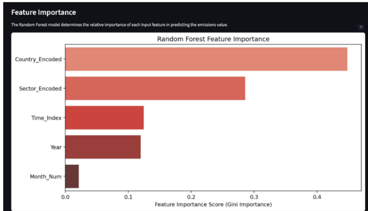
Figure 3.1: Random Forest feature importance for CO2 prediction
