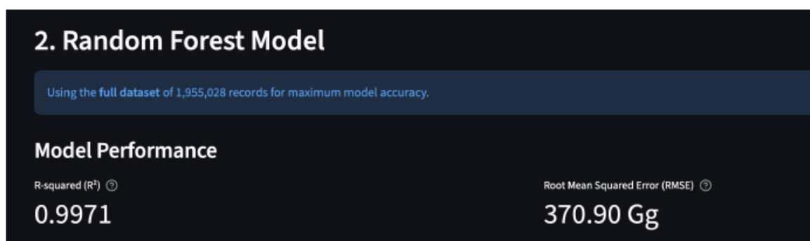
Figure 3.4: Random Forest performance with R^2 = 0.9971 and RMSE = 370.90 Gg
