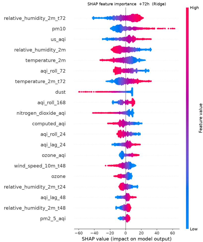
Figure 10. SHAP beeswarm at +72 h (Ridge). Colour encodes feature value; horizontal position encodes contribution to the prediction. Forecast humidity leads.
