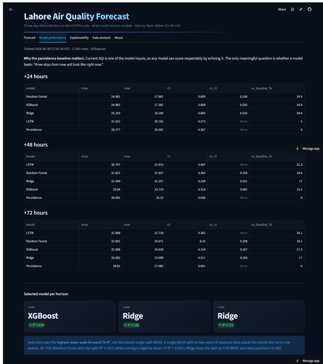
Figure 17. Model performance tab, showing every model against the persistence baseline and stating the selection criterion openly.
