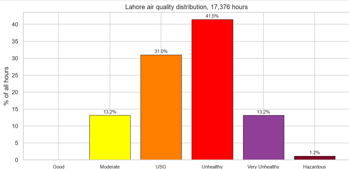
Figure 3. Distribution of hourly AQI across EPA categories. The 'Good' band is empty across the entire two-year record.
