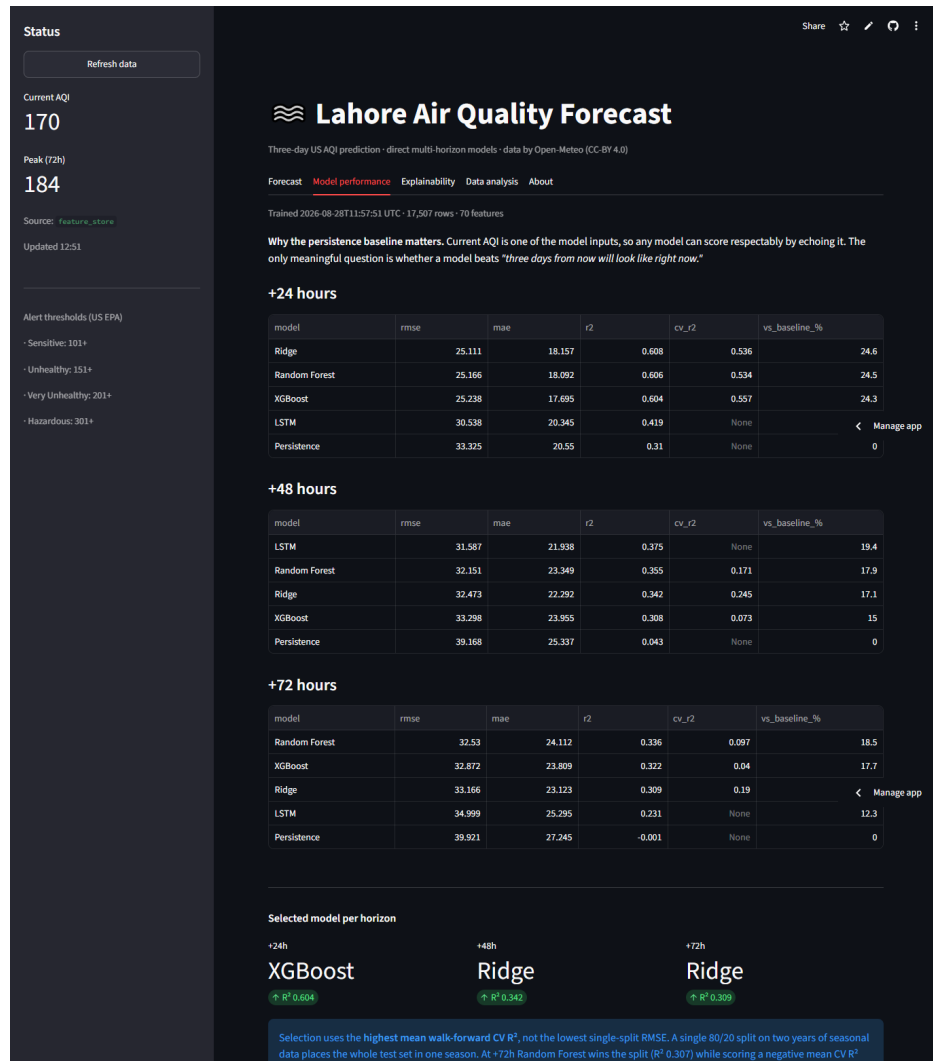
Figure 17. Model performance tab, showing every model against the persistence baseline and stating the selection criterion openly.
