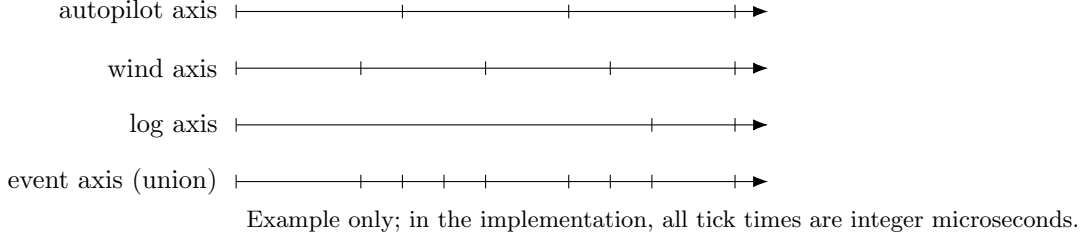
Figure 2: Multi-rate scheduling: each subsystem owns a time axis, and the engine integrates on their union (the event axis).
