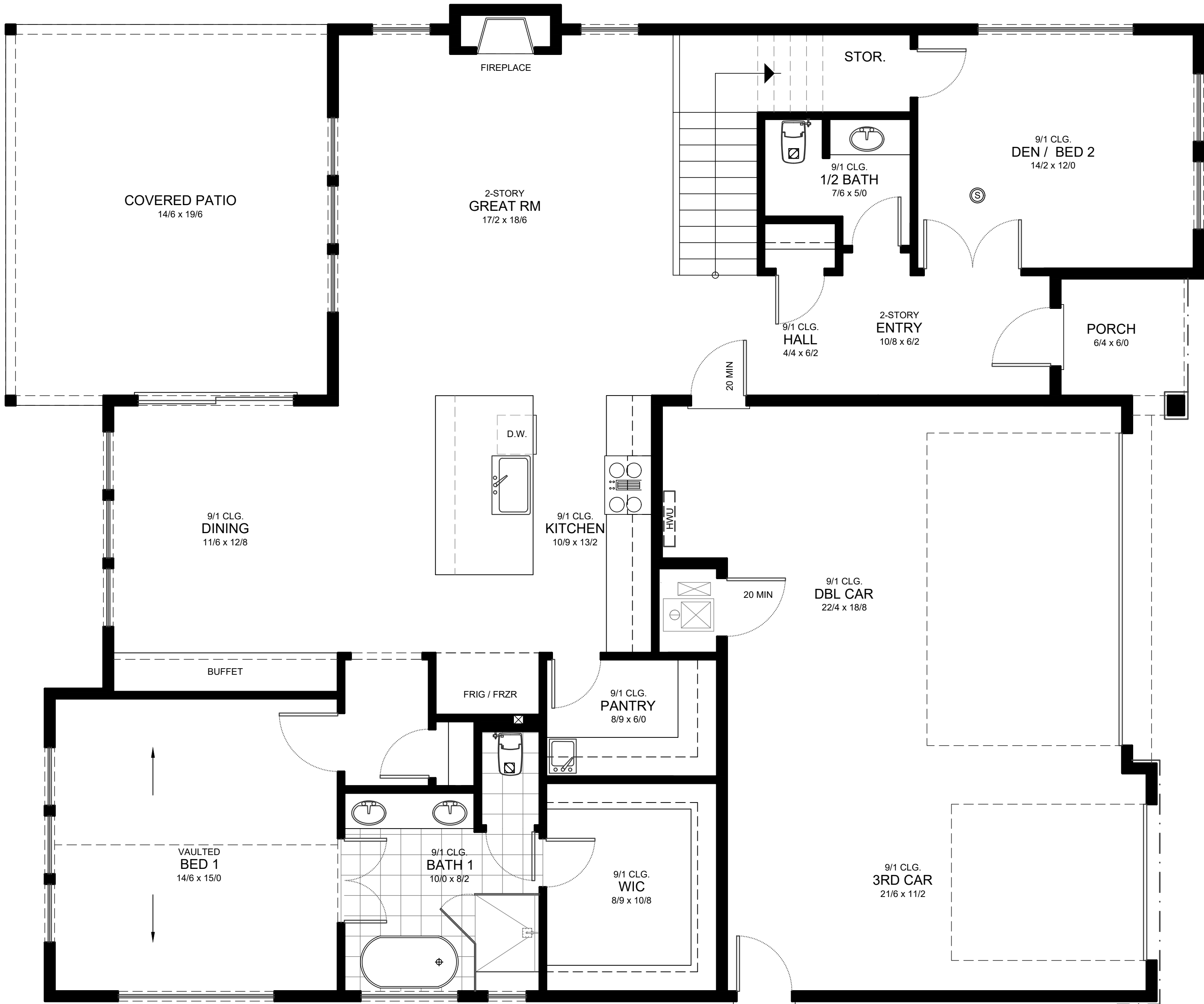
MAIN FLOOR PLAN SCALE: 1/4" = 1'-0"
