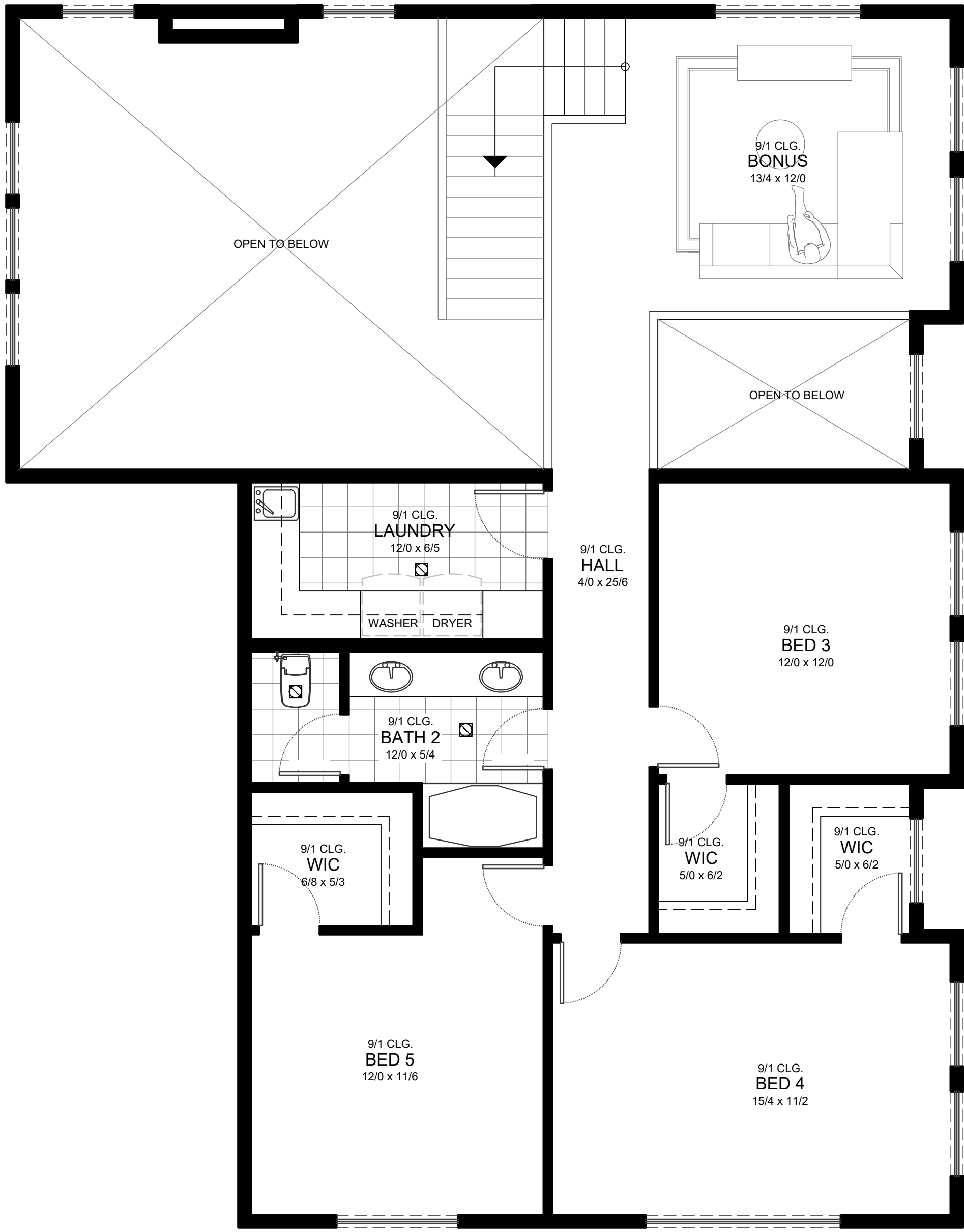
UPPER FLOOR PLAN SCALE: 1/4" = 1'-0"
