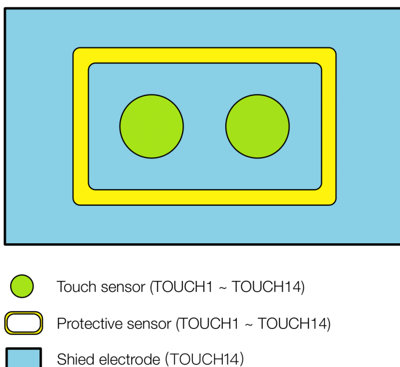
Fig. 19: ESP32-P4 Waterproof and Proximity Sensing Design
