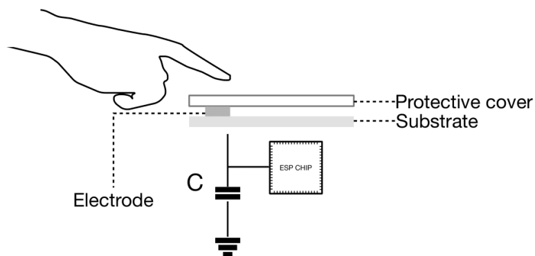
Fig. 16: ESP32-P4 Typical Touch Sensor Application
