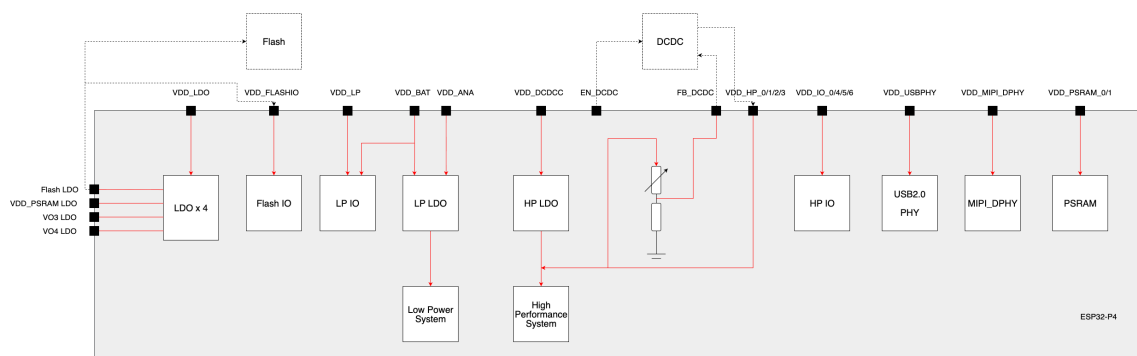
Fig. 3: ESP32-P4 Power Scheme
