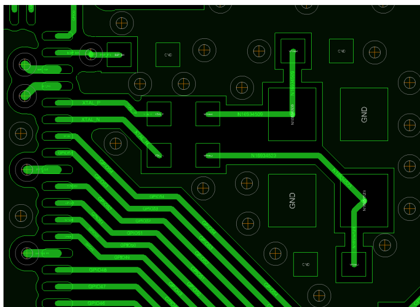
Fig. 15: ESP32-P4 Crystal Layout
