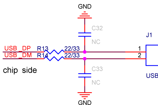
Fig. 13: ESP32-P4 USB RC Circuit
