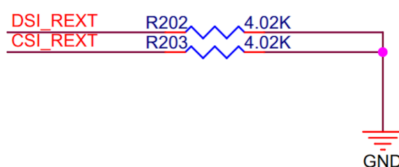
Fig. 14: ESP32-P4 Schematic for MIPI Signal
