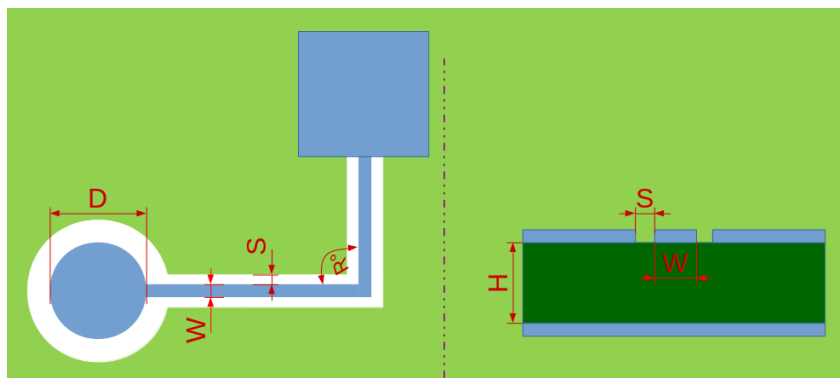
Fig. 18: ESP32-P4 Sensor Track Routing Requirements
