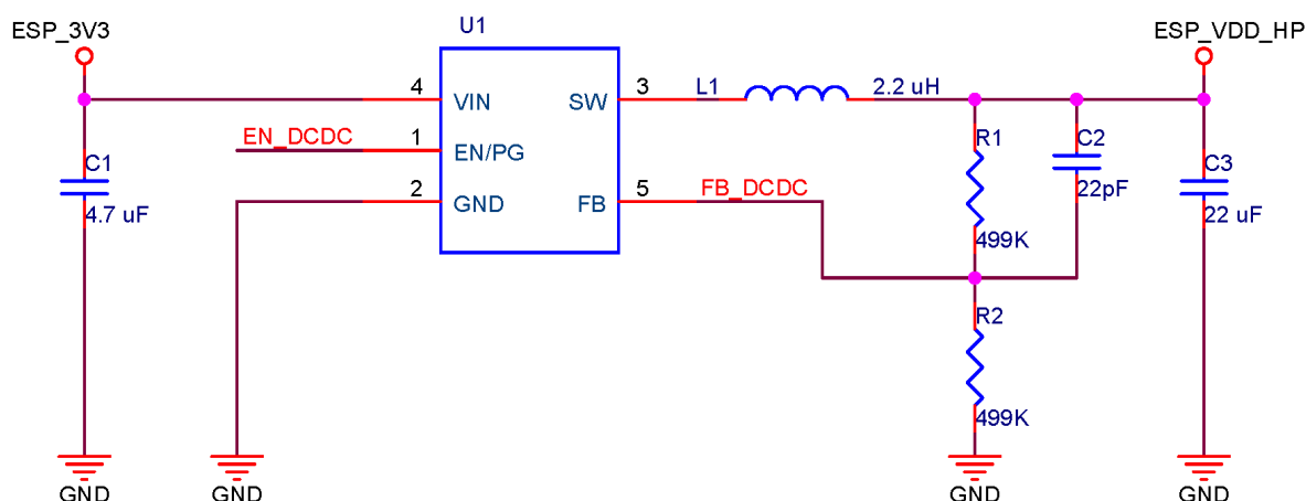
Fig. 5: TLV62569 Schematic (Chip Revisions v3.0 and Later)
