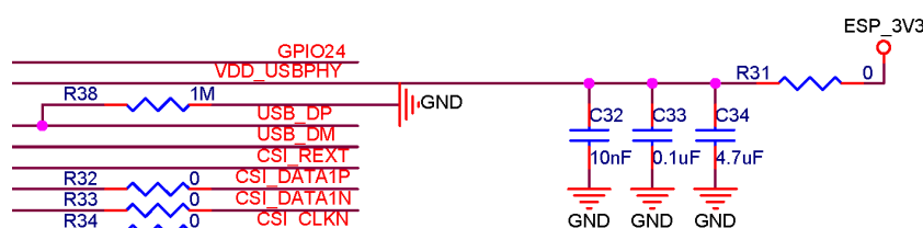
Fig. 12: DP Pull-down Resistor (Chip Revisions v1.0 and v1.3)
