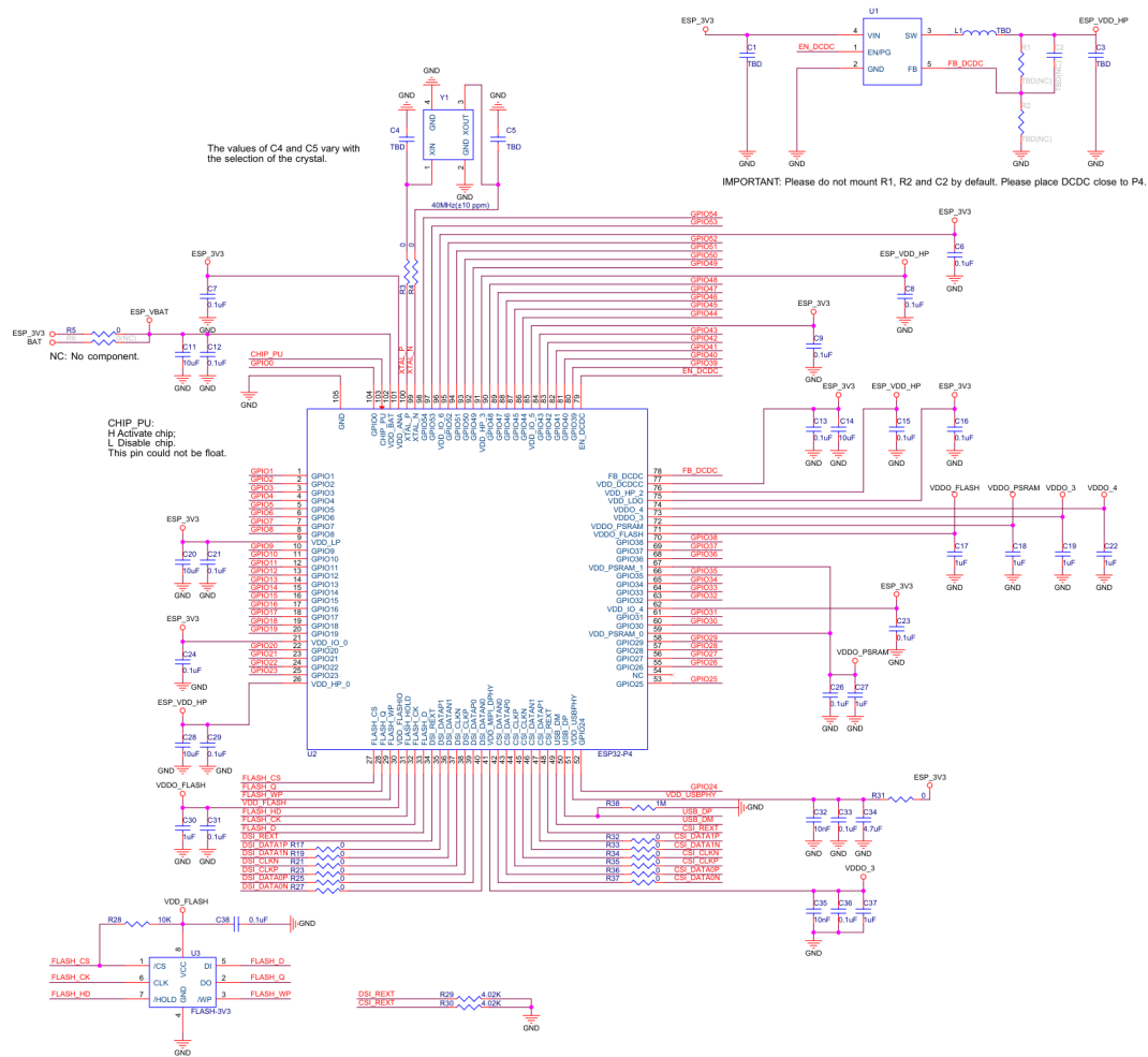
Fig. 2: ESP32-P4 Reference Schematic (Chip Revisions v1.0 and v1.3)
