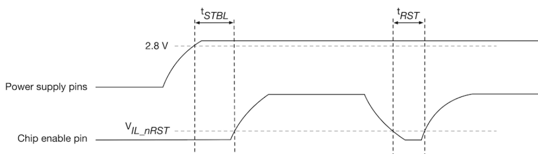
Fig. 7: ESP32-P4 Power-up and Reset Timing
