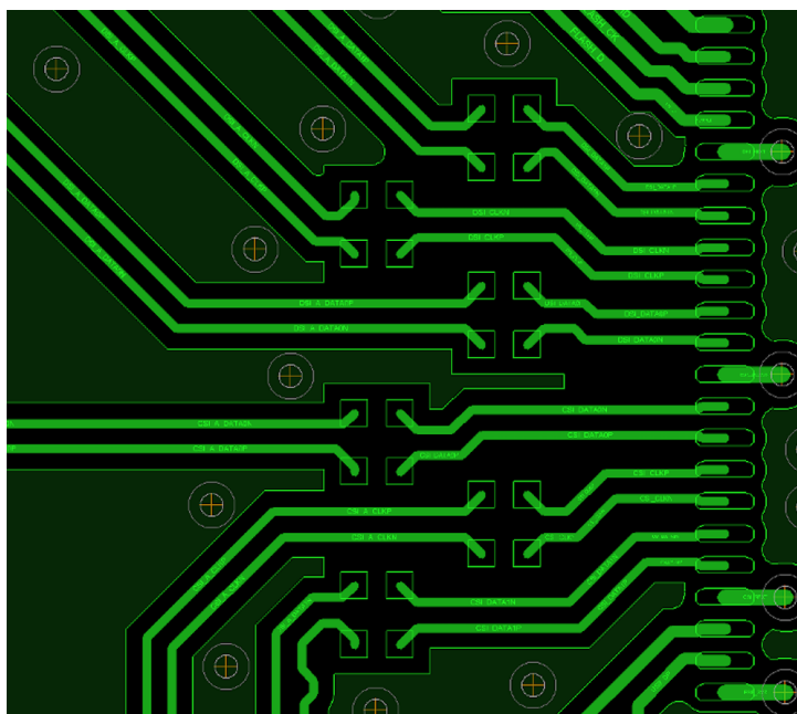
Fig. 20: ESP32-P4 MIPI Layout
