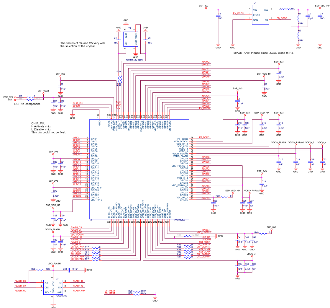
Fig. 1: ESP32-P4 Reference Schematic (Chip Revisions v3.0 and Later)
