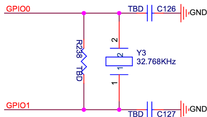
Fig. 9: ESP32-P4 Schematic for 32.768 kHz Crystal
