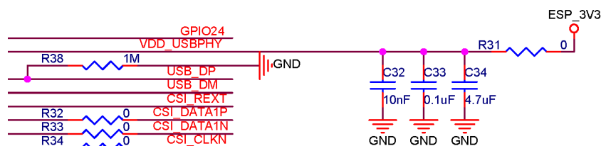
Fig. 4: VDD_USBPHY Reference Schematic (Chip Revisions v1.0 and v1.3)
