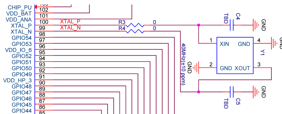
Fig. 8: ESP32-P4 Schematic for External Crystal
