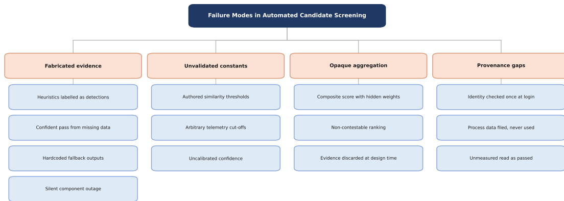
Fig. 5. Failure modes in automated candidate screening. The four families are not independent: fabricated evidence typically originates in an unvalidated constant and is concealed by opaque aggregation.
