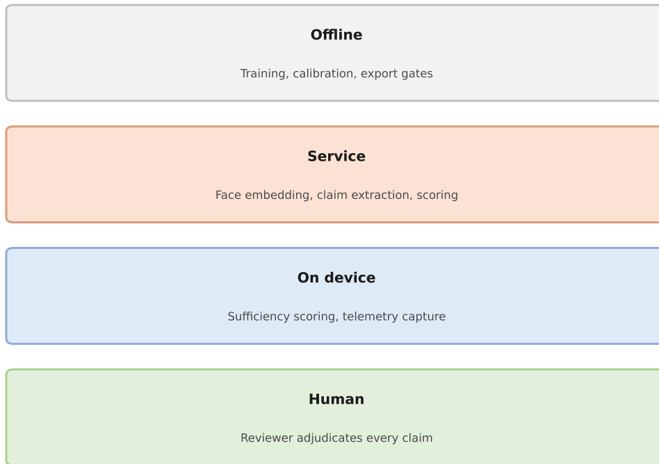
Fig. 17. Where each learned component runs. The human tier is not a fallback; it is the only tier that produces a decision about a person.
