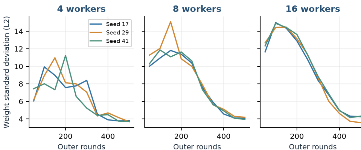
Figure 3. Exact weight standard deviation at the retained analysis cadence for the nine compressed AXL runs. Lines join measured points. Each scale shows all three seeds; lower late-training dispersion is consistent with the decaying learning rate.
