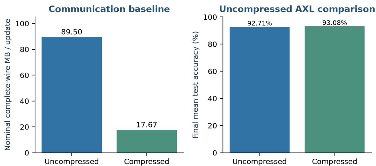
Figure 2. Left: nominal complete-wire bundle sizes from accepted compression accounting, in decimal MB. Right: the W4 seed-17 uncompressed AXL comparison and matching compressed AXL final mean accuracies. The accuracy axis starts at zero.
