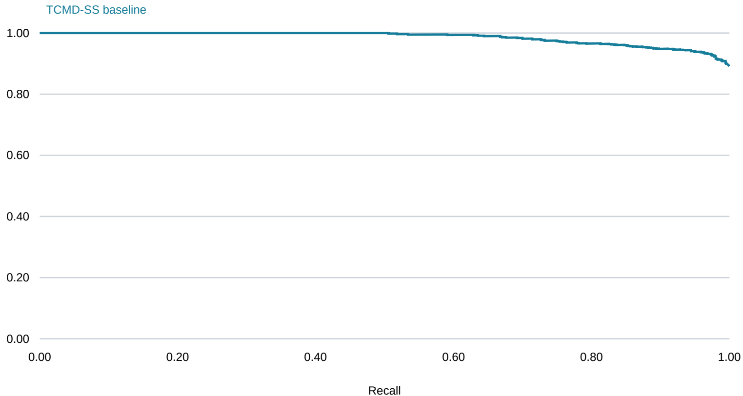
Figure 2. Historical development precision-recall
