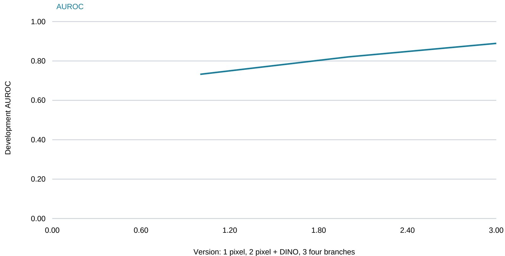
Figure 4. Shared-checkpoint scoring ablations
