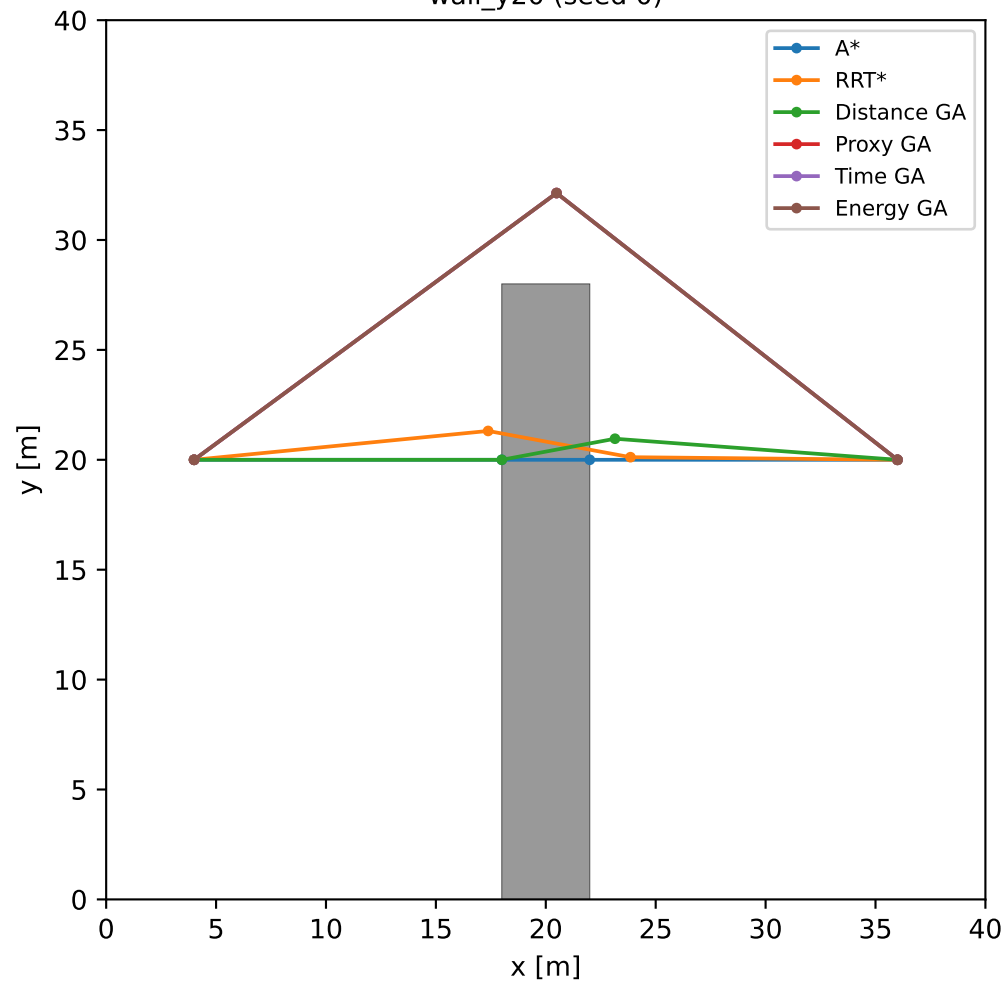
wall_y20 (seed 0)
