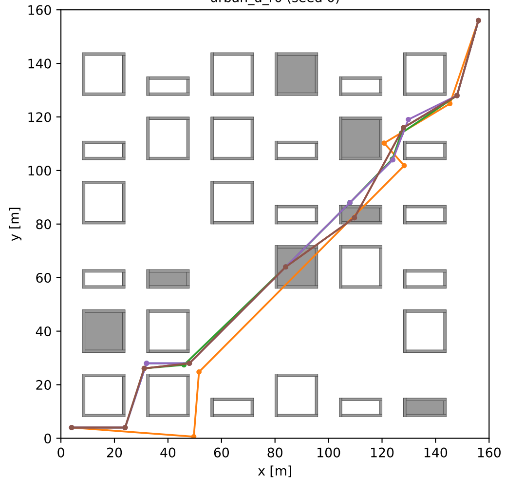
urban_a_r0 (seed 0)
