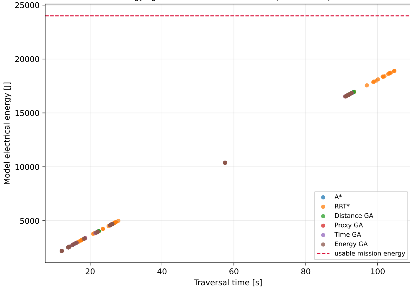
Energy against traversal time, all development attempts
