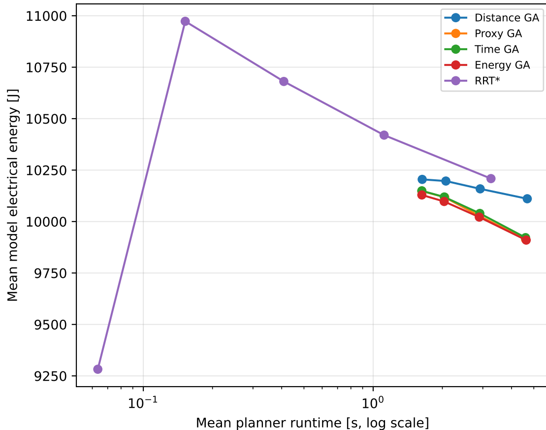
Quality against runtime
