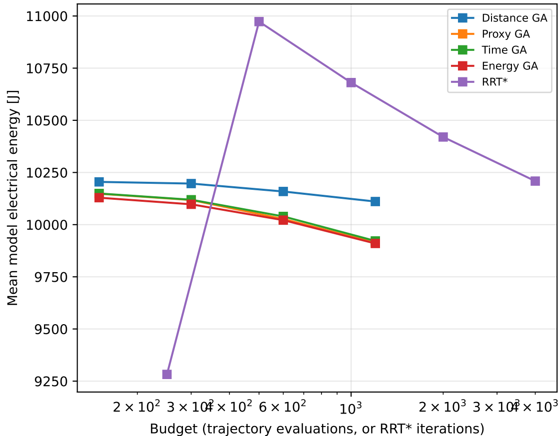
Quality against matched budget
