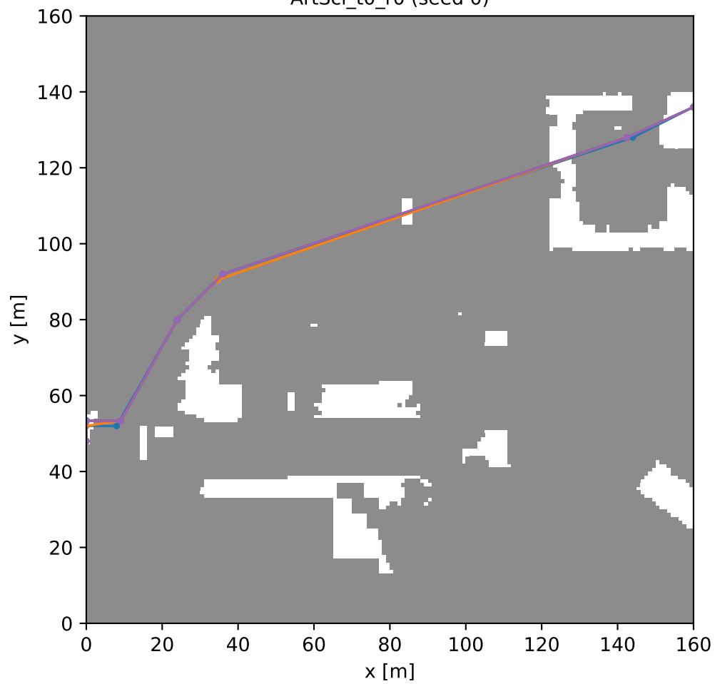
ArtSci_t0_r0 (seed 0)
