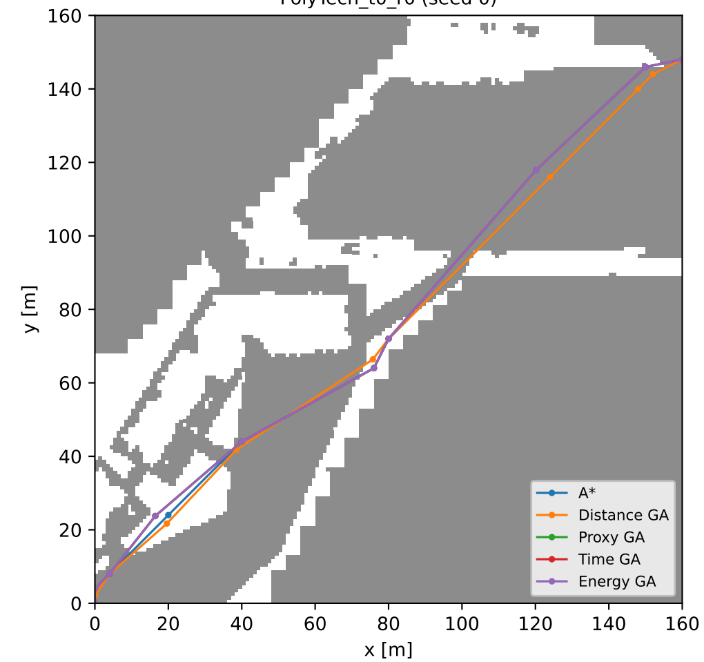
PolyTech_t0_r0 (seed 0)
