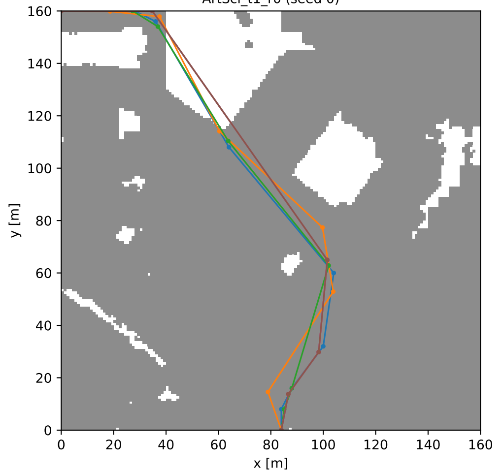
ArtSci_t1_r0 (seed 0)
