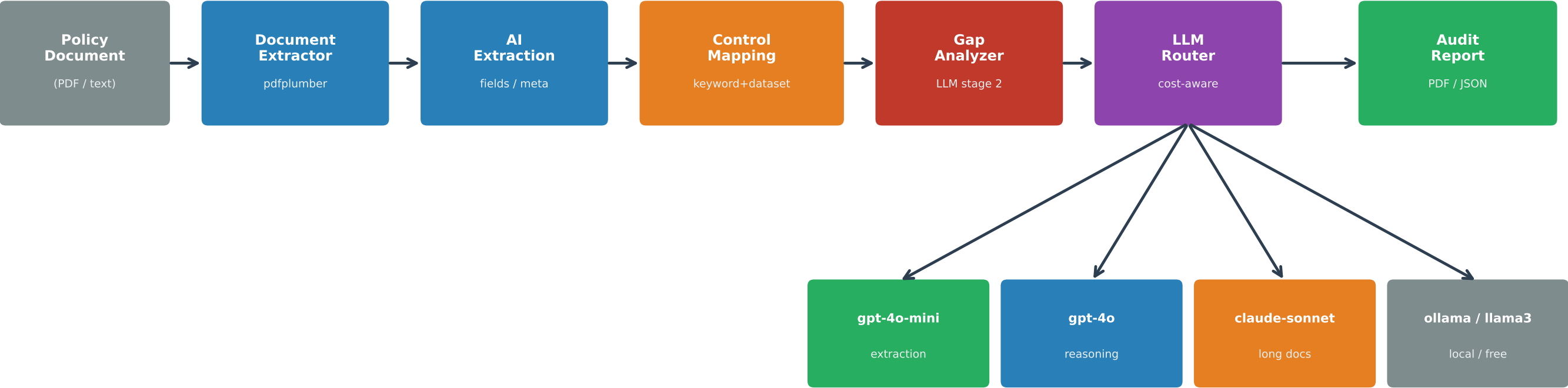
LLM Models
