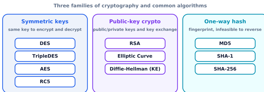
Figure 9.5: Three families of cryptography
