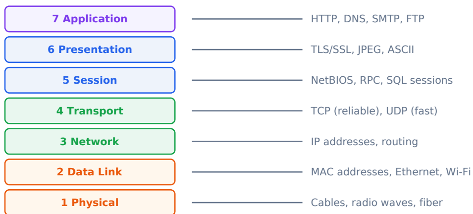
Figure 7.5: The OSI model
