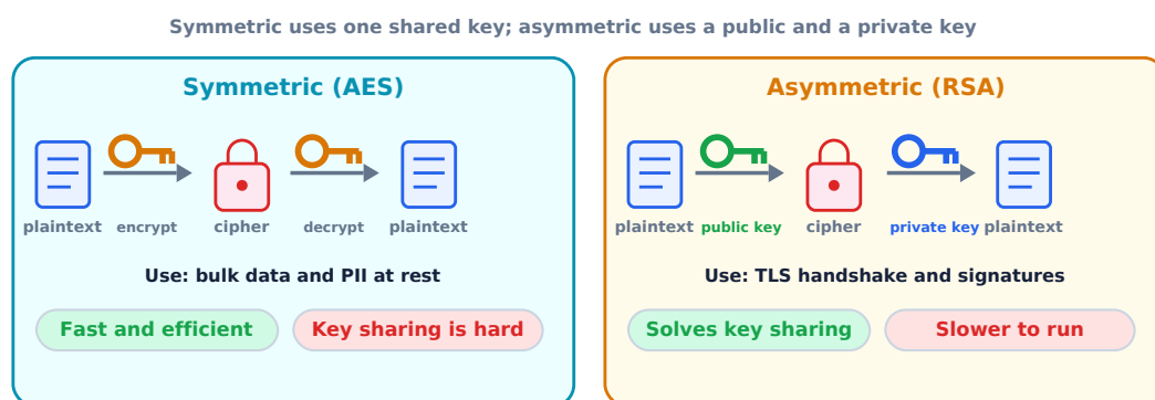
Figure 4.5: Symmetric versus public-key encryption
