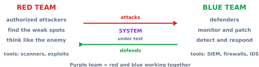
Figure 6.1: Red team versus blue team
