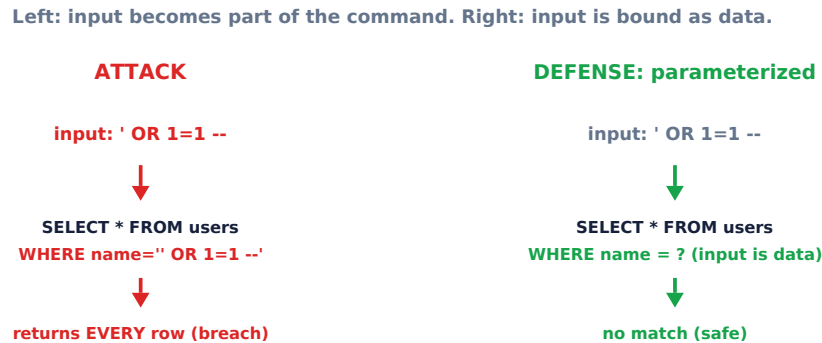
Figure 10.3: SQL injection vs a parameterized query
