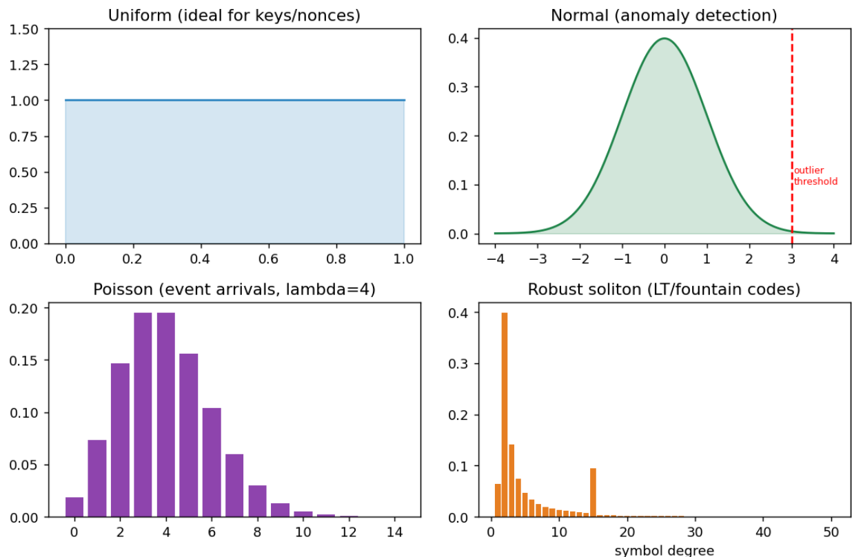
Figure 58: Uniform, normal, Poisson, and robust soliton probability distributions compared
