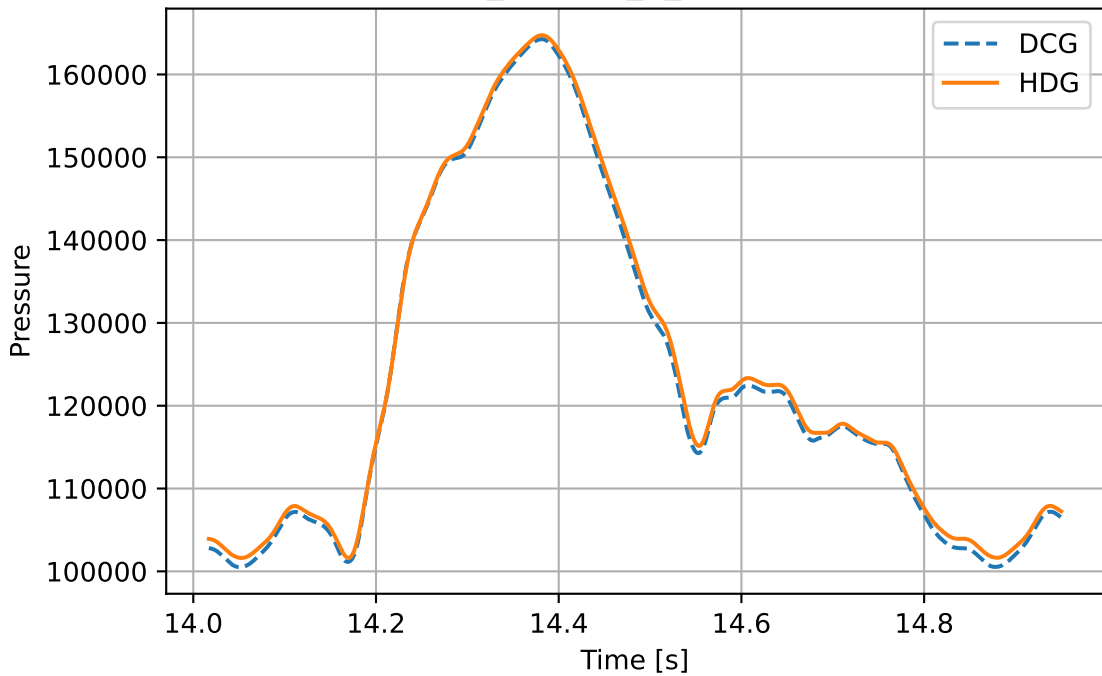
iliac_femoral_R_II Pressure
