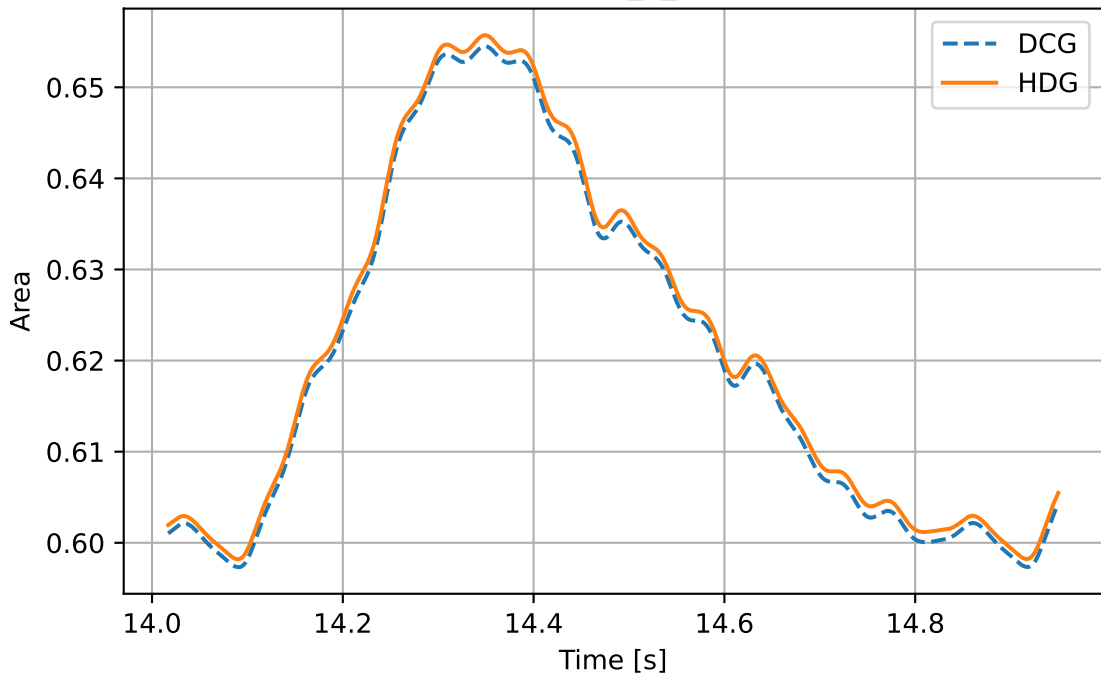
subclavian_L_I Area
