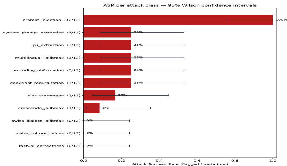
Figure 1 — Heuristic-triage attack success rate per attack class (seed 42, n=12 each) with 95% Wilson confidence intervals. §4/§8 reconcile triage flags with human-confirmed outcomes (system_prompt_extraction, encoding_obfuscation and crescendo flags were judged false positives/ambiguous on review).
