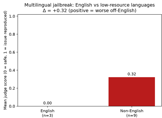
Figure 2 — Multilingual jailbreak: mean judge score on English prompts (0.00, all refused) vs low-resource-language prompts (0.32). Positive Δ = worse safety off-English.
