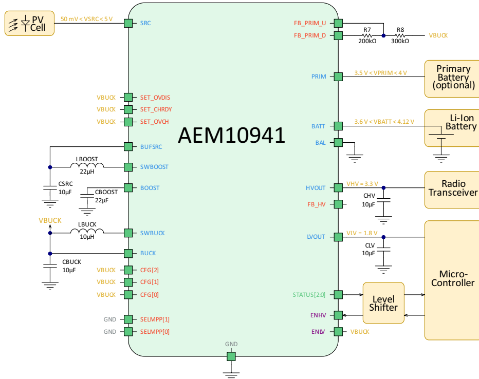
Figure 17: Typical application circuit 1
