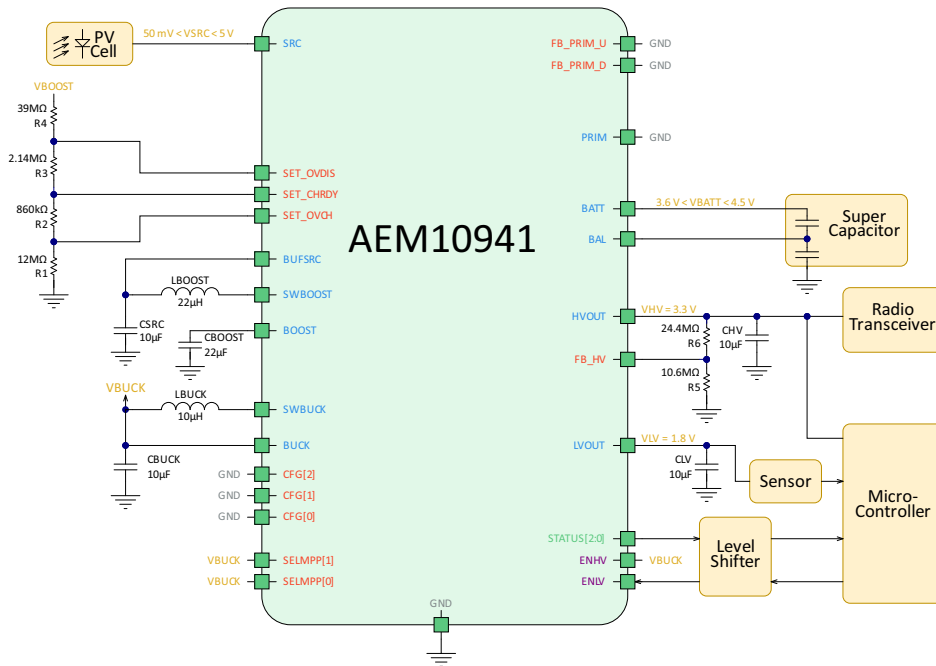
Figure 18: Typical application circuit 2
