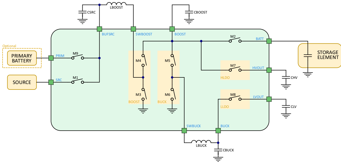
Figure 12: Simplified schematic view of the AEM10941
