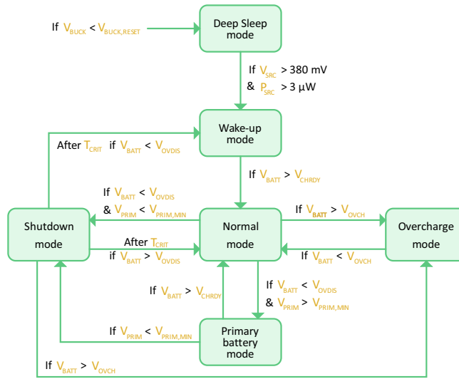
Figure 13: Diagram of the AEM10941 modes
