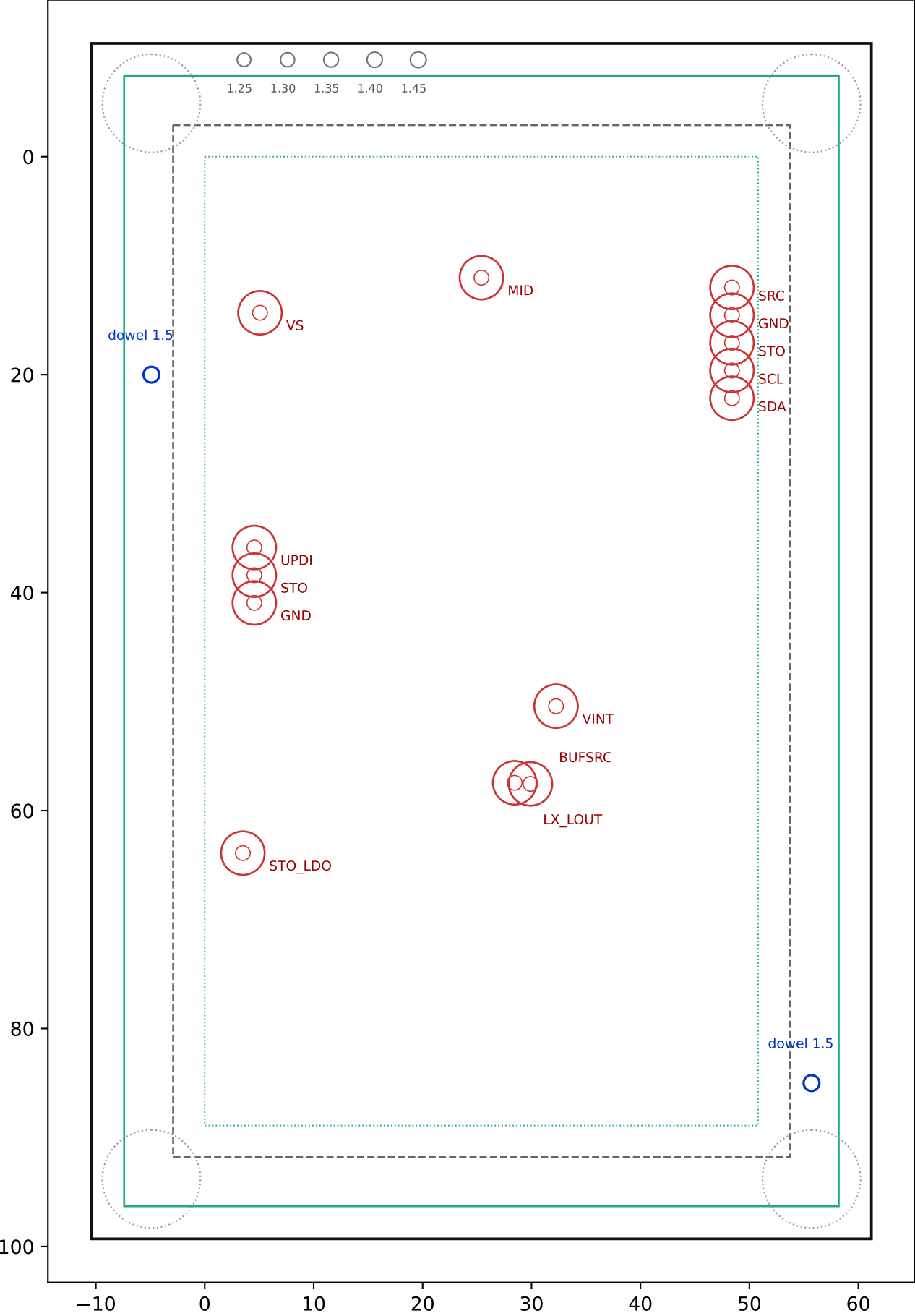
POGO TEST PLATE — top view, board coordinates (green: panel / card; red: probe bosses)
