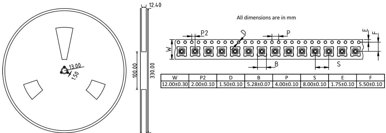
Figure 25: Tape and reel dimensions
