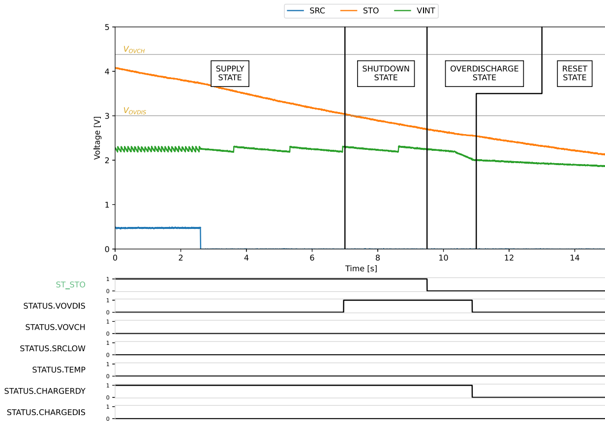
Figure 18: Overdischarge behavior
