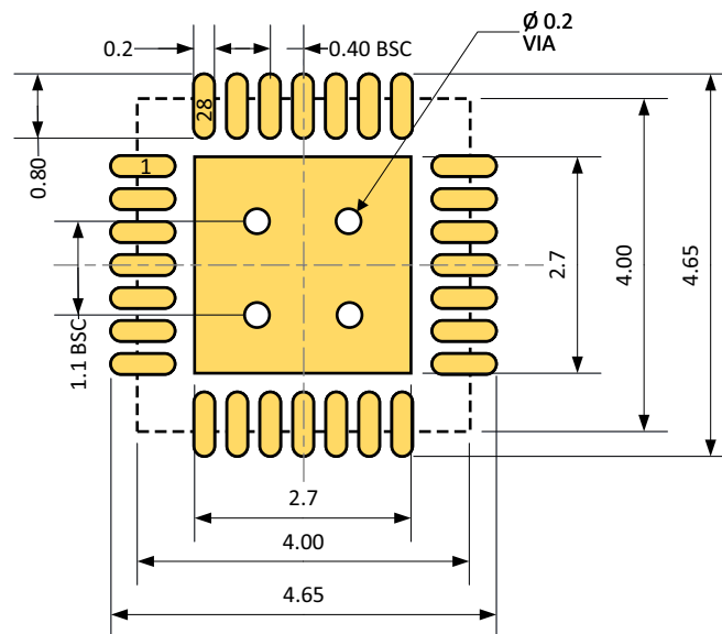
Figure 27: Recommended board layout for QFN28 package (all dimensions in mm)
