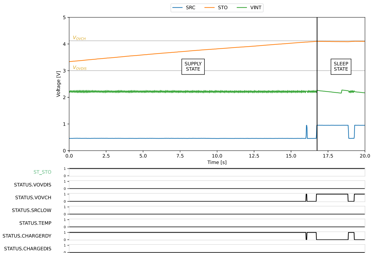
Figure 17: Supply and overcharge behavior
