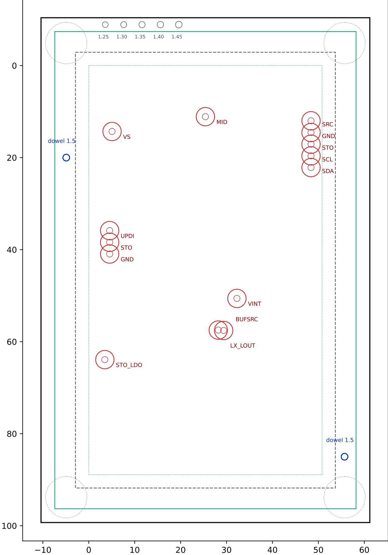
POGO TEST PLATE — top view, board coordinates (green: panel / card; red: probe bosses) Z stack / build notes
