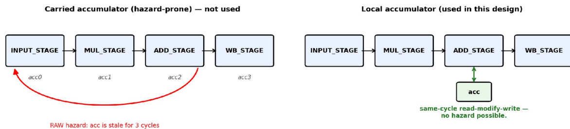
Figure 2: Carried vs. local accumulator
