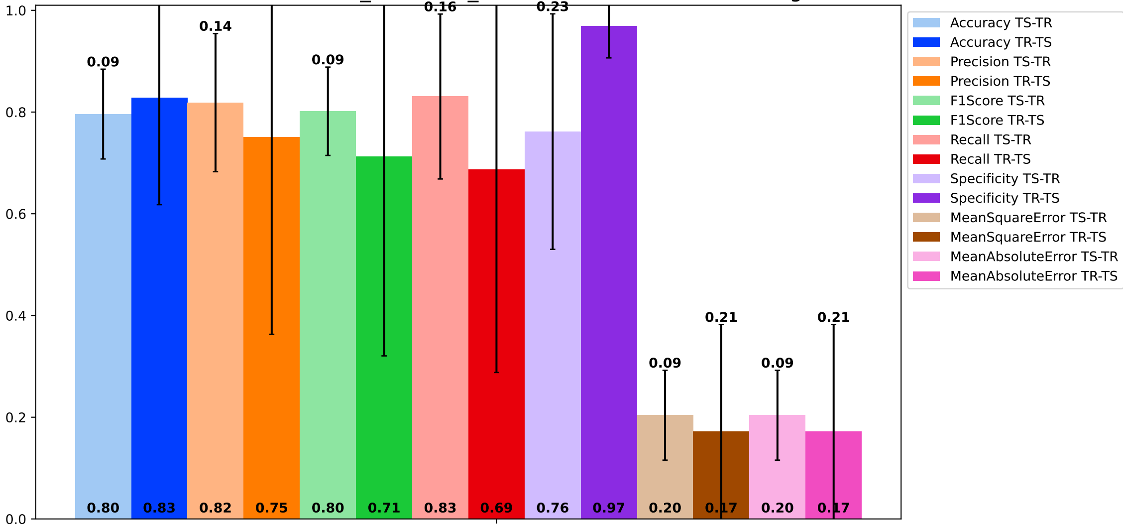
adversarial - reduced_balanced_androcrawl - GradientBoosting
