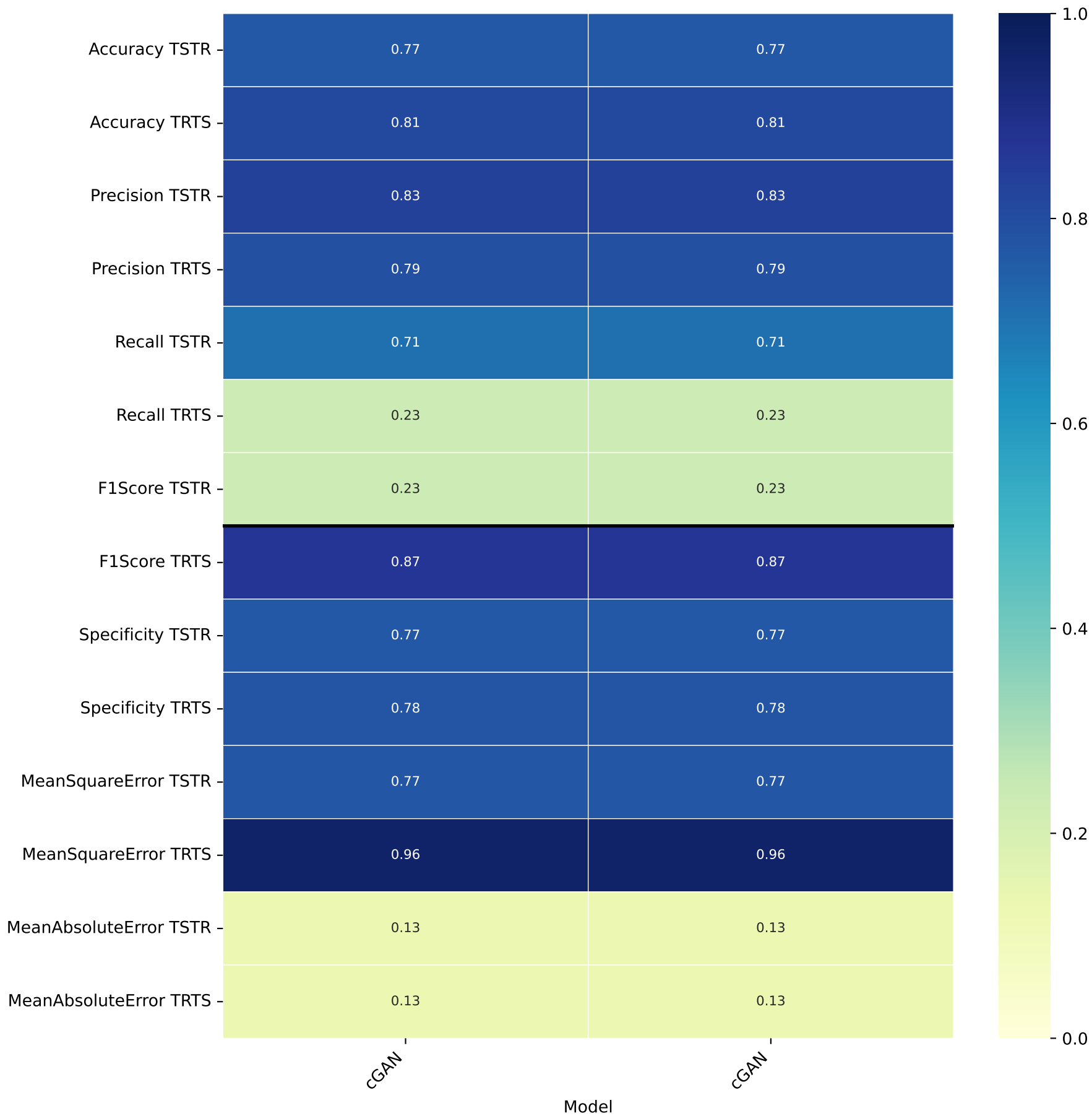
SVM performance utility_across_models
