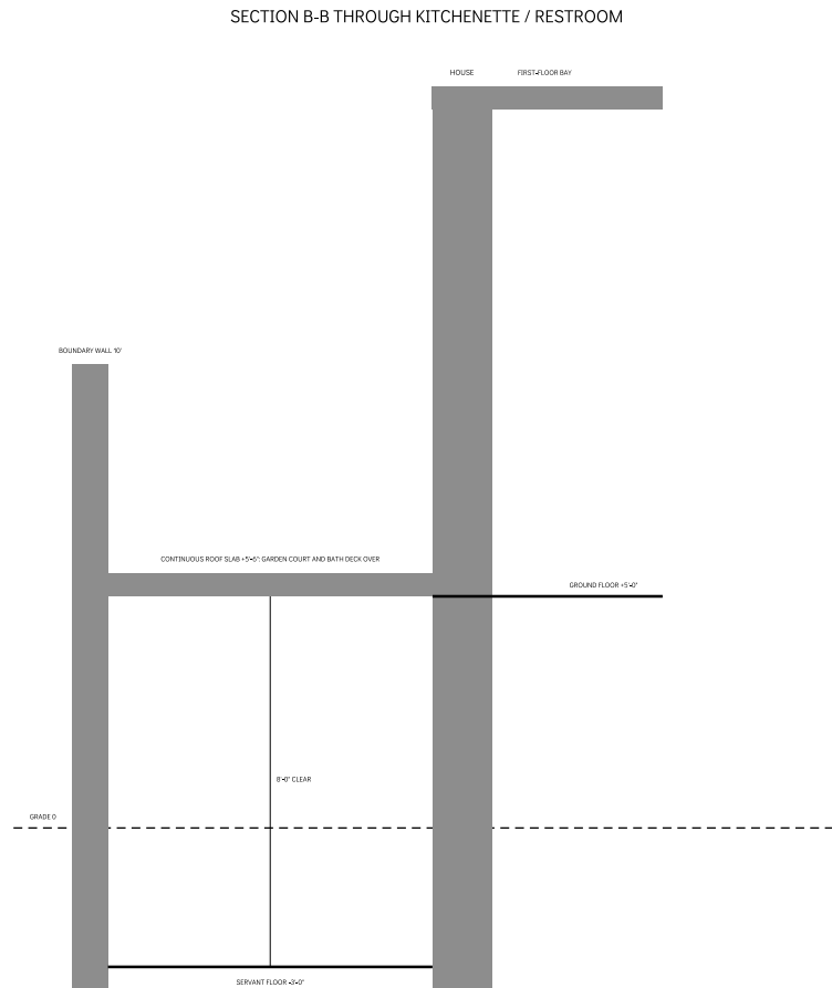
SECTION B-B THROUGH KITCHENETTE / RESTROOM
