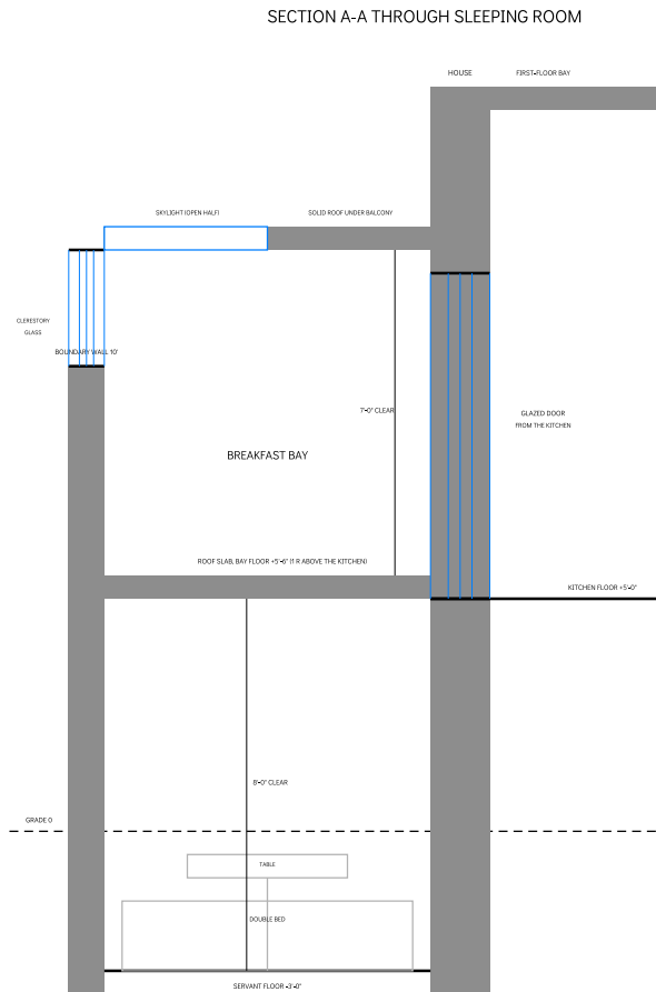
SECTION A-A THROUGH SLEEPING ROOM
